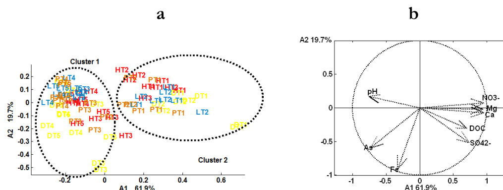
Fig. 5 : first principal plan of principal component analysis performed for As, Fe, Ca, NO 3 - , pH, SO 4 2- , Mg and DOC concentrations of the 80 rhizosphere solution samples. Representation of cluster groups on the first plan (a) and relationship between As and measured parameters (b) for the two first principal components (1-Axis versus 2-Axis). Rhizosphere solution samples were identified by the code “XTy” where “X” means H: H. lanatus (red), D: D. viscosa (yellow), L: L. corniculatus (blue) or P: P. lanceolata (orange) and “Ty” means T1, T2, T3, T4 and T5).
