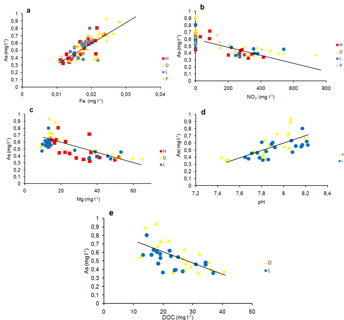
Fig. 6 : As concentration ( \text{mg L}^{-1} ) as a function of (a) Fe concentration ( \text{mg L}^{-1} ) for all studied species ( r=0.76^* ) (□ : Control; ■ : H. lanatus ; ▲ : D. viscosa ; ● : L. corniculatus ; +: P. lanceolata ), (b) \text{NO}_3^- concentration ( \text{mg L}^{-1} ) for all selected species ( r=-0.72^* ), (c) Mg concentration ( \text{mg L}^{-1} ) for H. lanatus , D. viscosa and L. corniculatus ( r=-0.67^* ), (d) pH value for D. viscosa and L. corniculatus ( r=0.65^* ) and (e) DOC concentration ( \text{mg L}^{-1} ) for D. viscosa and L. corniculatus ( r=-0.6^* ).
