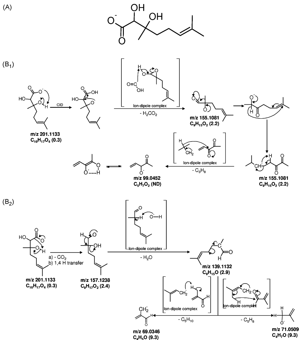
Fig. 6. (A) Structure proposed by CAS for the unknown metabolite at m/z 201.1133 ( C_{10}H_{18}O_4 ) and putative predictive fragmentation mechanisms B1: starting with a neutral loss of H_2CO_2 and B2: starting with a neutral loss of CO_2 . Exact masses and masses error on formula determination (ppm) are indicated under each product ion (ND = not detected).
