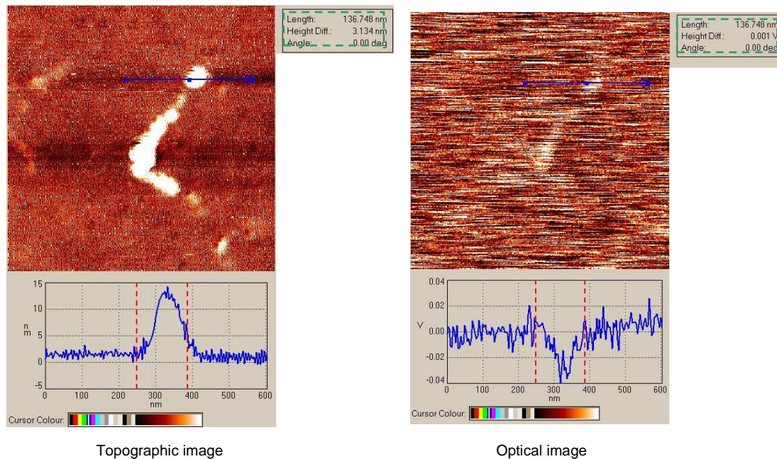
Figure III- 21: SNOM topographic and optical images of hybrid nanoparticles with respective line profiles.
