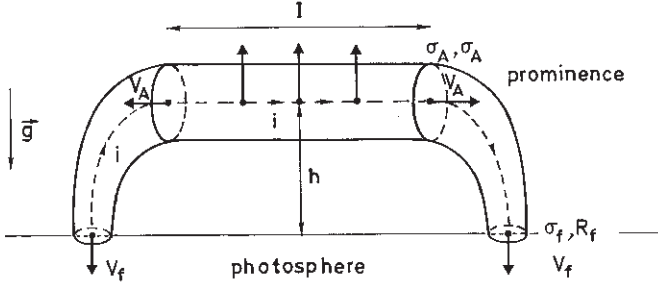
Fig. 8. Flux rope model
