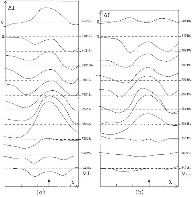
Fig. 6a and b. Variation of \Delta I(\Delta\lambda) for 2 points of the filament versus time. a and b correspond to points 1 and 2 of Figs. 3 and 4, and arrows indicate the centre of the profiles
