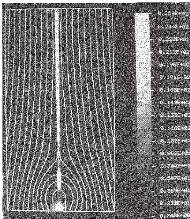
FIGURE 4a : Same as above (mass density in grey levels), but for t=151.2 \tau_a . A Kippenhahn-Schlüter prominence has formed at the top of the closed magnetic loops at the base of the box (they are obtained by reconnection). A Kuperus-Raadu prominence has formed around and above the X neutral line location. In this case, we used \tau_R/\tau_a=20 .
