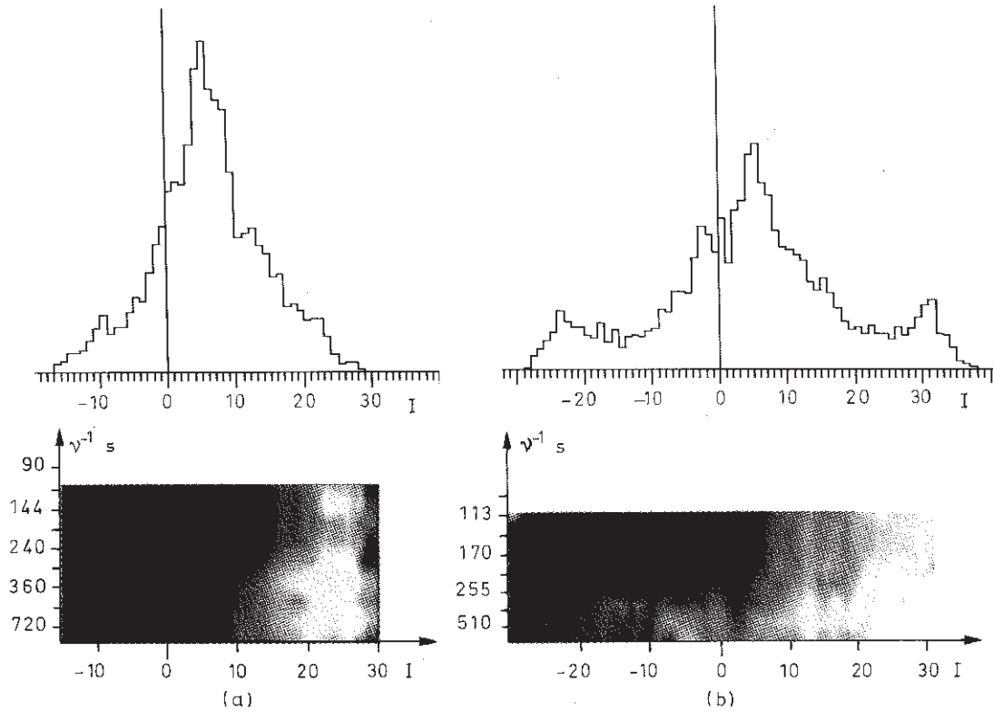
Fig. 4a and b. H \alpha intensity-distribution function and 2D diagram (I, \nu) for velocity power spectrum on a 1980, September 30 and b 1980, September 28. The intensity I is a mean value over the time sequence for each pixel
