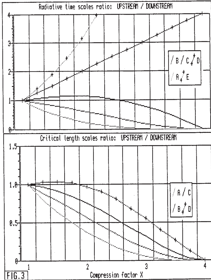
Figure 3, Top panel: The ratio \tau_{Ru}/\tau_{Rd} as a function of \chi for different values of \alpha (A: -2.5, B: -1.0, C: 0.0, D: 1.0, E: 1.8), corresponding to different temperature ranges. Bottom panel: The ratio L_{cu}/L_{cd} as a function of \chi for different \alpha values (A: -2.5, B: -1.0, C: 0.0, D: 0.9).
