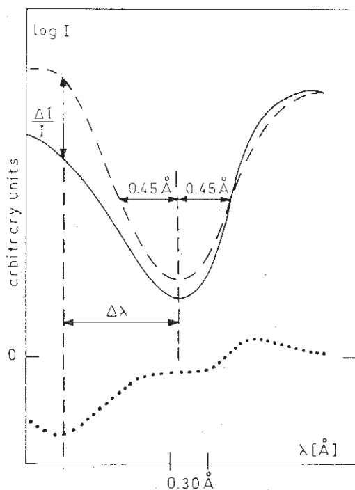
Fig. 3. 'Cloud model' interpretation of line profiles in the filament: mean chromospheric profile I_0(\lambda) , - - - - -; observed current profile I(\lambda) , ———; [I(\lambda) - I_0(\lambda)]/I_0(\lambda) , ······. The intensity \Delta I and velocity V_c of the cloud are reported.
