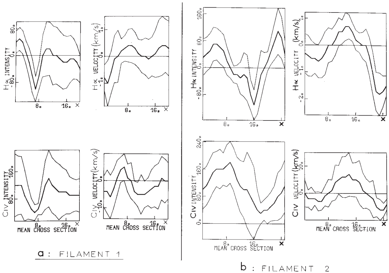
Fig. 3 a and b. Intensities I and velocities \bar{V} across filaments, averaged along y direction parallel to their long axis. In abscissae: x direction perpendicular to y (in units of 3 arcsec) in ordinates: mean intensity I or mean velocity \bar{V} in H \alpha or C IV (thick lines), plus or minus the standard deviation ( \sigma_I or \sigma_V (thin lines). Intensities are measured in arbitrary units, and velocities in \text{km s}^{-1} . a Filament of box 1 (28 September). b Filament of box 2 (2 October)
