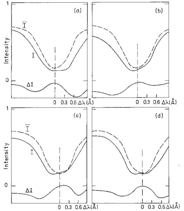
Fig. 5a-d. H\alpha profiles I(\Delta\lambda) of 4 points in the filament at 8:02:19 UT (thick lines). The mean chromospheric profile \bar{I}(\Delta\lambda) is represented in dashed lines, and below, the difference between them \Delta I(\Delta\lambda) = I(\Delta\lambda) - \bar{I}(\Delta\lambda) is displayed. a-d correspond to points 1, 2, 3, 4 indicated on Figs. 3 and 4
