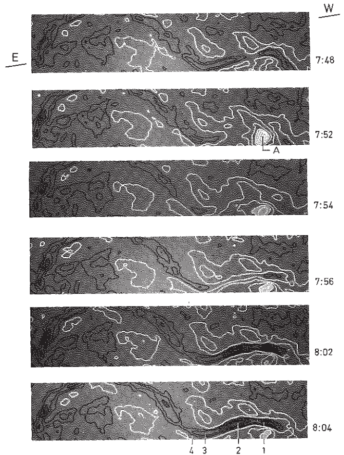
Fig. 3. H\alpha intensity isocontours ( H\alpha \pm 0.3 \text{ \AA} ) at different times (UT). White lines correspond to bright features (step=100 in arbitrary units) and black lines to dark features (step=50 in arbitrary units)
