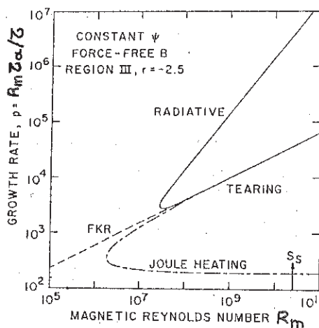
Dependence of the growth rates of various modes on the magnetic Reynolds number. The dashed curve is the FKR tearing-mode solution, the short-long dashed curve is the present solution without radiation, and the solid curve is the present solution with both radiation and Joule heating.
