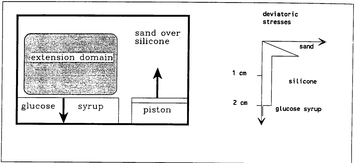
Fig. 15: Top view of the experimental apparatus and the rheological profile used.
