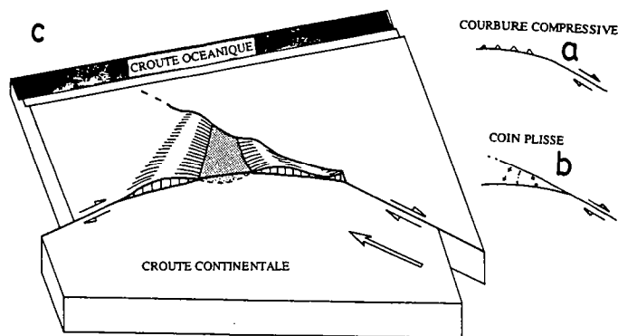
FIG. 7. - Bloc diagram of a «folded wedge» structure.
