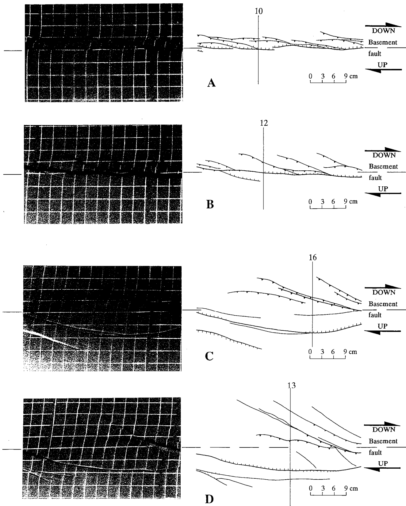
Fig. 4 - 19. Photographs and line drawings of faults developed with the same oblique-slip (5 cm) and same strike-slip/dip slip ratio ( SS/DS = 3,5 ), above a 90^\circ basement fault, with different rheologies
