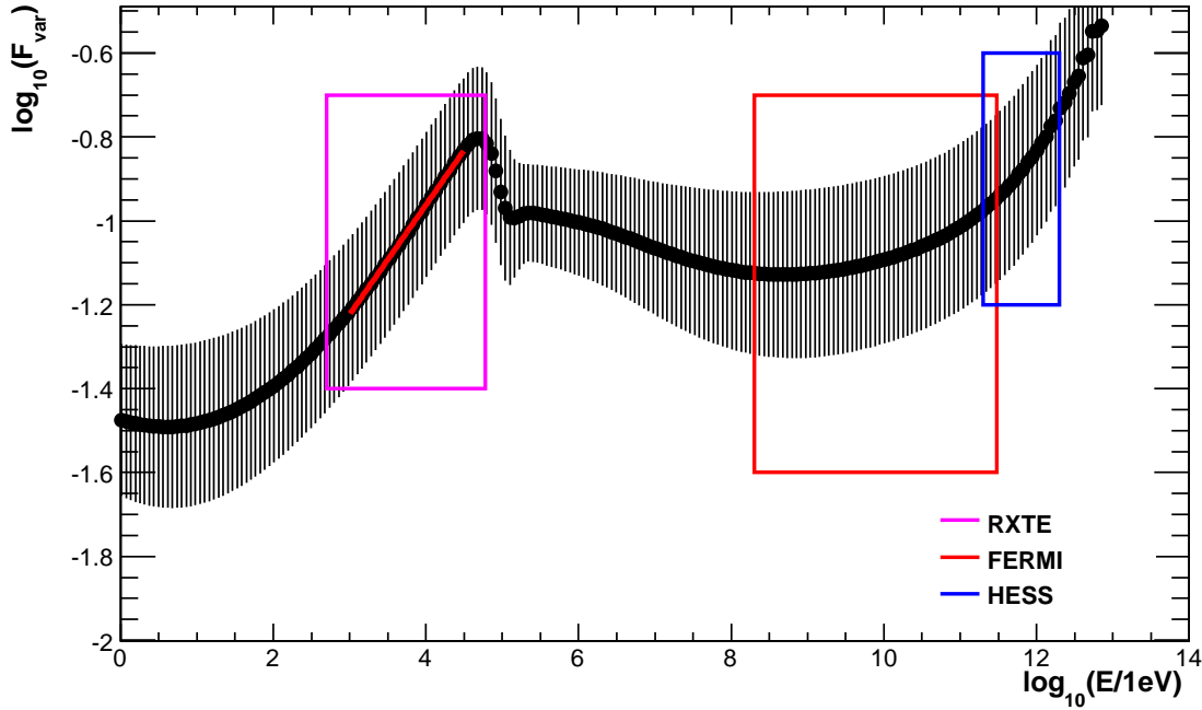
Figure 3.7: The spectral variability distribution (SVD) using a time-dependent SSC model where a maxwellian electron distribution is injected using a red noise time profile.
