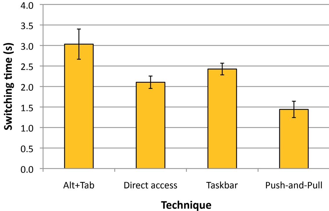
Figure 4.7: Mean switching time for SWITCHING TECHNIQUE. Error bars represent 95% confidence interval.
