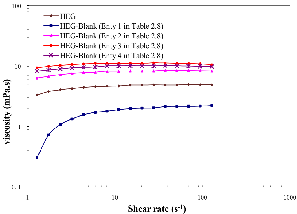
Figure 2.15: Variation of the viscosity as a function of shear rate for some samples of HEG derivatives from blank experiments in water at a concentration of 4.8 g/L at 25 °C.
