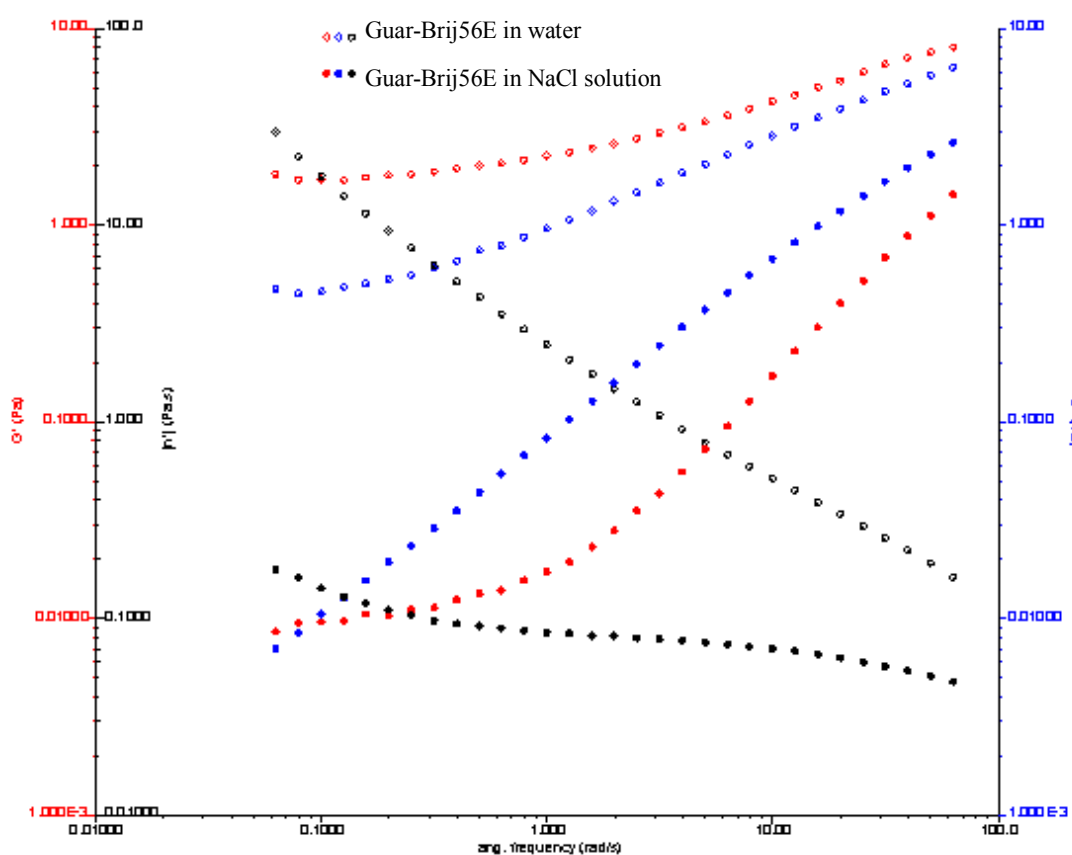
Figure 2.12: Comparison of the storage and loss moduli as a function of frequency for solutions of Guar-Brij56E (4.8g/L) in pure water and in 0.1 M NaCl at 25 °C.
