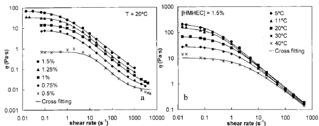
Figure 1.14: Steady state curves of HMHEC aqueous solutions a) at T = 20^\circ\text{C} and several concentrations; b) at [\text{HMHEC}] = 1.5\% and several temperatures. 99
