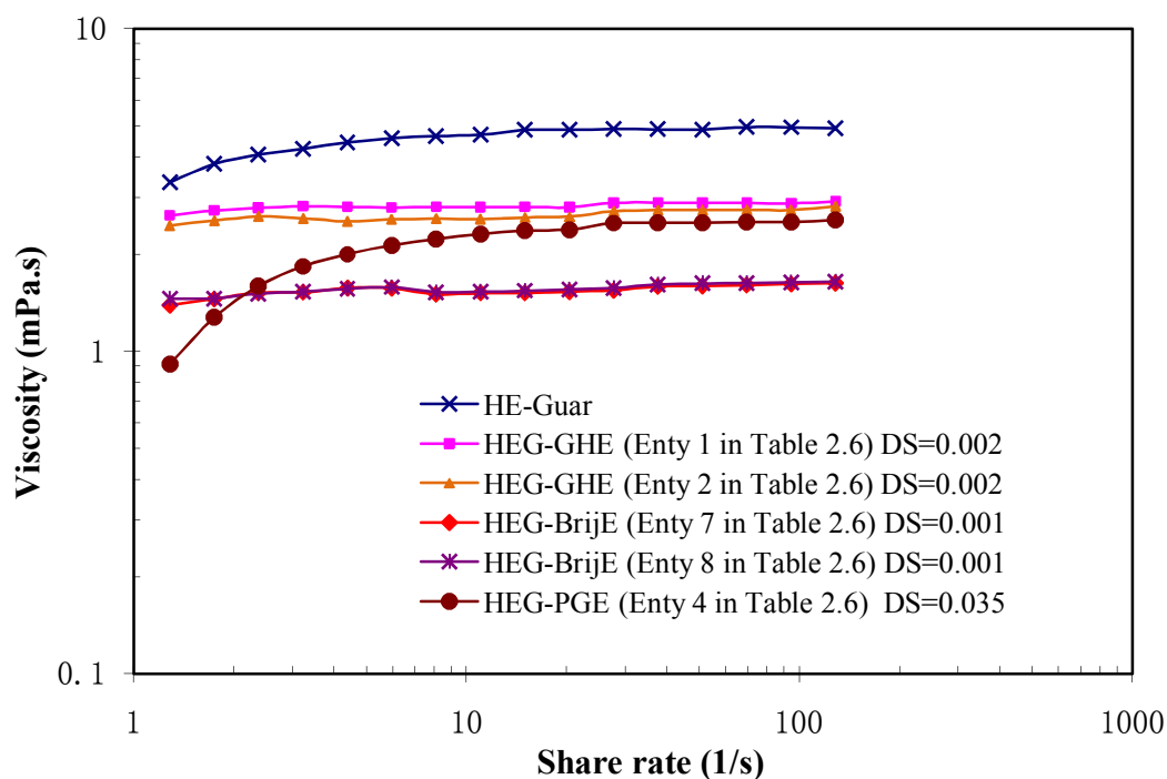
Figure 2.13: Variation of the viscosity as a function of shear rate for some samples of HEG derivatives in water at a concentration of 4.8 g/L at 25 °C.
