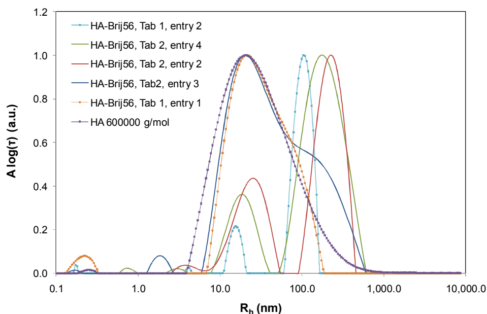
Figure 3.3: Analysis of HA-Brij56E derivatives in PBS ( C_p = 2 g/L) by dynamic light scattering. Angle fixed at 90° and temperature fixed at 25 °C. (Tab 1 is Table 3.1, Tab 2 is Table 3.2,)
