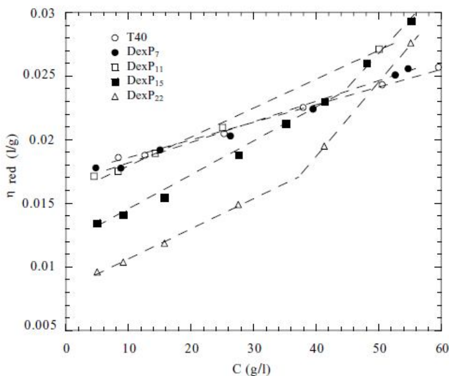
Figure 1.17: Variation of the reduced viscosity of aqueous solutions of dextran T40 and hydrophobically modified dextrans (water, 25°C). 34
