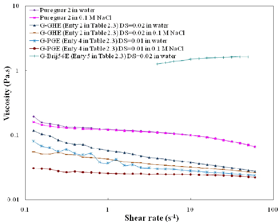
Figure 2.7: Variation of the viscosity as a function of shear rate for some samples of guar derivatives in water and in aqueous solution of NaCl (0.1 M) at a concentration of 4.8 g/L at 25 °C.
