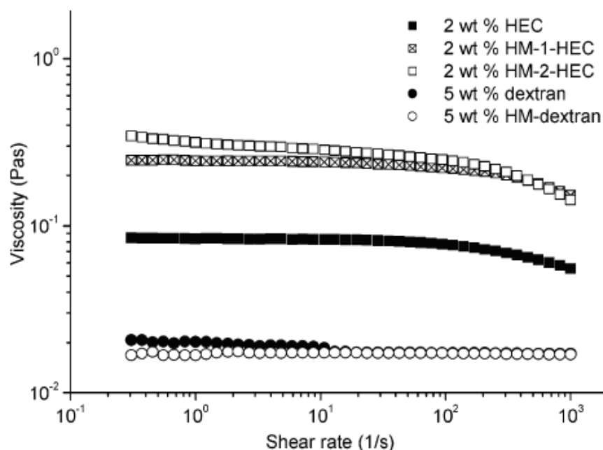
Figure 1.13: Shear rate dependence of the viscosity in 1 M NaOH for 2 wt % solutions of HEC, HM-1-HEC, and HM-2-HEC and for 5 wt % solutions of dextran and HM-dextran. 94
