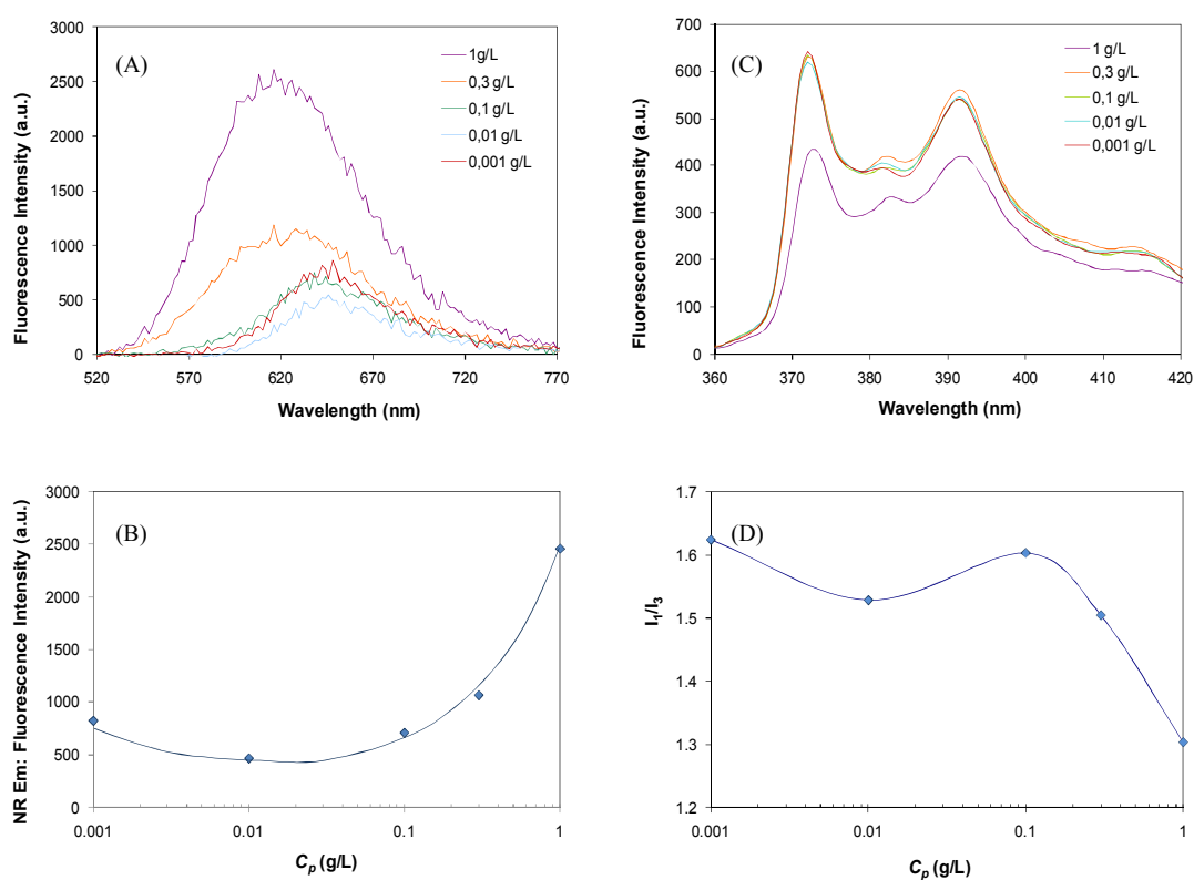
Figure 3.4 : Analysis of the self-assembly of HA-Brij56E by fluorescence spectroscopy: area-normalized fluorescence emission ( \lambda_{\text{ex}}=505 nm) spectra of Nile red ( 1.5 \times 10^{-6} M) in the HA-Brij56E /PBS system as a function of HA-Brij56E concentration obtained for reaction conditions of Table 3.1, entry 2, as an example (A,B); fluorescence emission ( \lambda_{\text{ex}}=336 nm) spectra of pyrene ( 3 \times 10^{-6} M) in the
