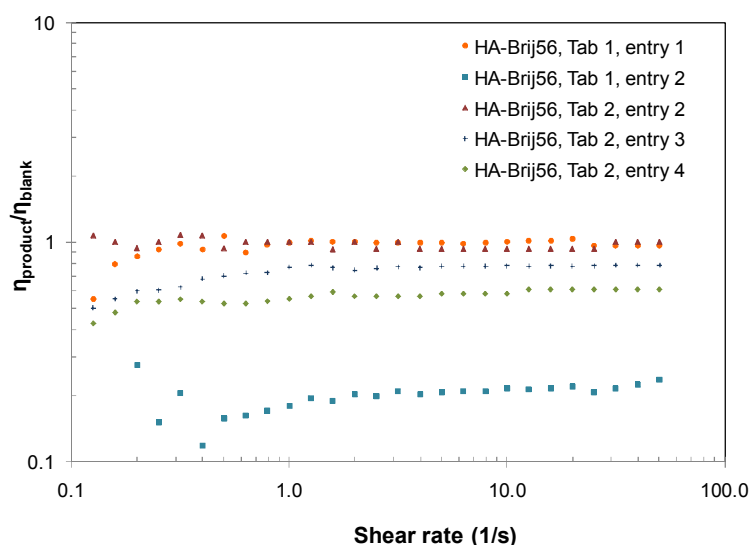
Figure 3.2: Variation of the viscosity of HA-Brij56E derivatives (10 g/L in PBS) divided by that of “their blank” as a function of shear rate. Temperature: 25 °C. (Tab 1 is Table 3.1, Tab 2 is Table 3.2,)
