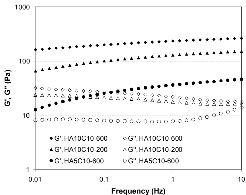
Fig. 1.19: Comparison of the storage and loss moduli as a function of frequency for solutions of decylaminohydrazide derivatives of HA in PBS at 25 °C and at a polymer concentration of 10 g/L. The derivatives are designated as HAxC 10 , x reflects the degree of substitution (DS; x = 100 DS) of the decyl (C 10 ) chains. 109
