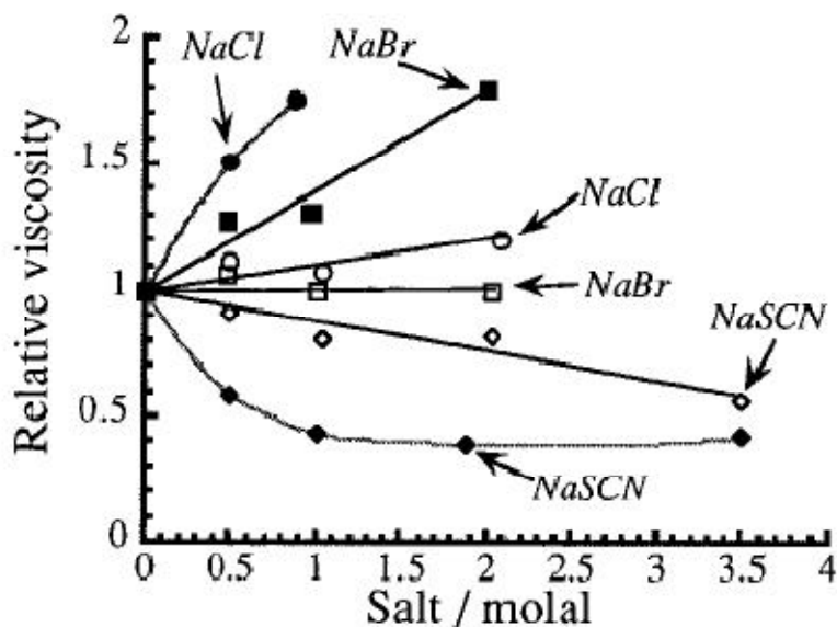
Figure 1.16: Relative viscosity of a 1 % (w/w) EHEC solution (open symbols) or a 1% (w/w) HM-EHEC solution (filled symbols) as a function of added NaCl (○, ●), NaBr (□, ■), or NaSCN (◇, ◆). 103
