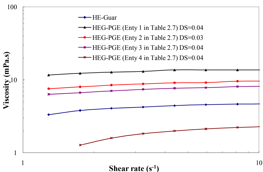
Figure 2.14: Variation of the viscosity as a function of shear rate for some samples of HEG derivatives in water at a concentration of 4.8 g/L at 25 °C.
