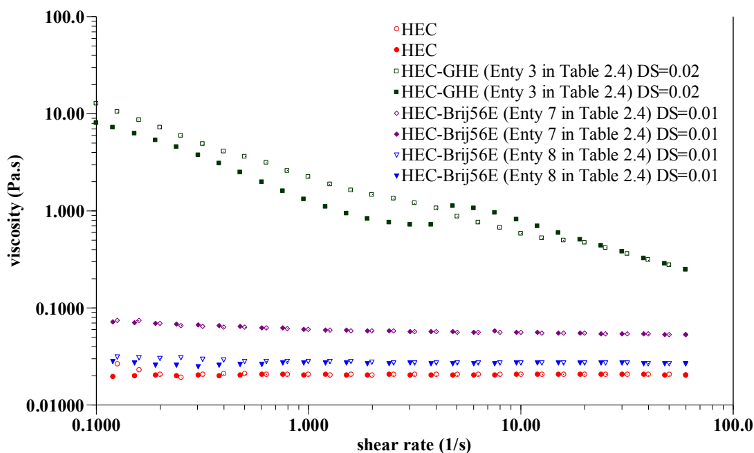
Figure 2.10: Variation of the viscosity as a function of shear rate for some samples of HEC derivatives in water at a concentration of 25 g/L at 25 °C. Open symbols: curves obtained from increasing shear rates; closed symbols: curves obtained from decreasing shear rates.
