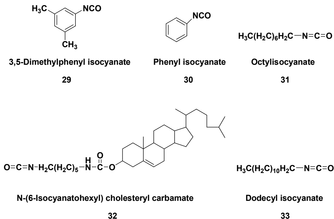
Figure 1.11: Isocyanate reagent.
