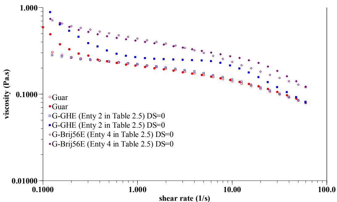
Figure 2.11: Variation of the viscosity as a function of shear rate for some samples of guar derivatives in water at a concentration of 4.8 g/L at 25 °C. Open symbols: curves obtained from increasing shear rates; closed symbols: curves obtained from decreasing shear rates.
