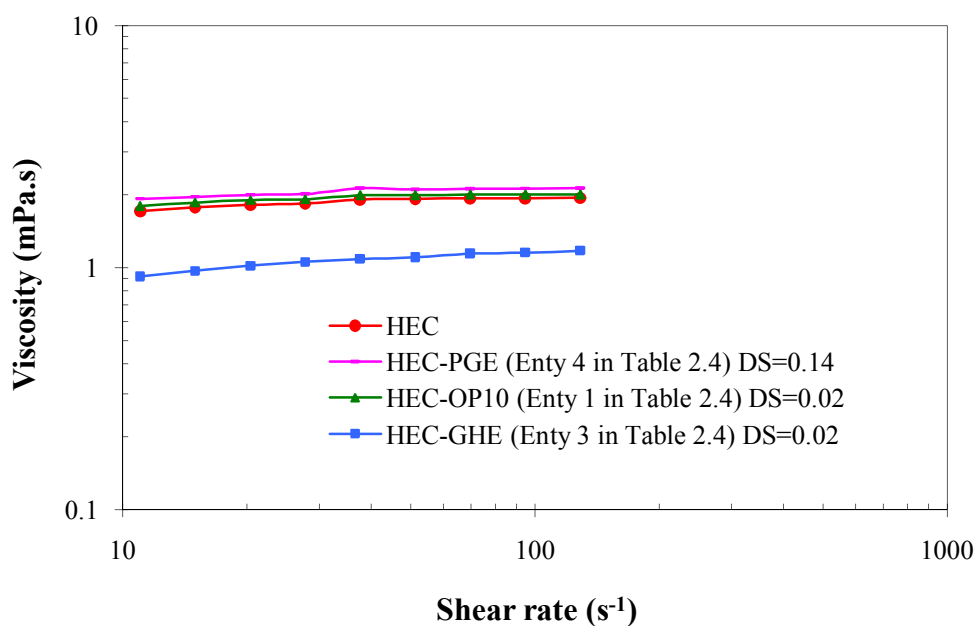
Figure 2.9: Variation of the viscosity as a function of shear rate for some samples of HEC derivatives in water at a concentration of 4.8 g/L at 25 °C.
