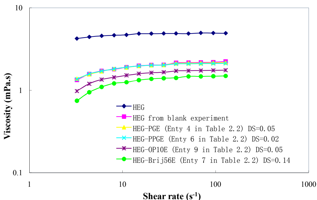
Figure 2.6: Variation of the viscosity as a function of shear rate for some samples of HEG derivatives in water at a concentration of 4.8 g/L at 25 °C.
