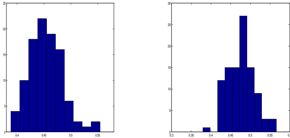
FIGURE 2.2 – Histograms of \hat{D}_N and \tilde{D}_N for 100 samples of FARIMA(1, d , 1) with D = 0.5 for N = 10^5 .
