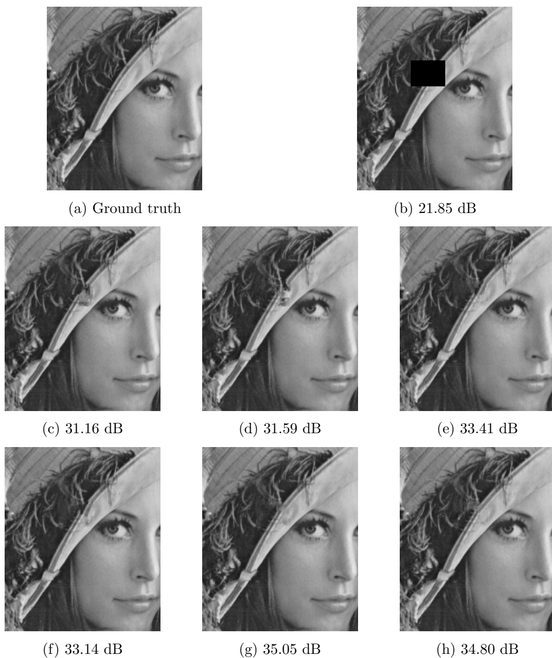
Figure 6.7: Missing region completion PSNR results for Lena image - (a) Ground truth image, (b) inpainting mask, (c) TM with priority of [43], (d) TM with augmented priority, (e) ATM with augmented priority, (f) NLM with augmented priority, (g) NMF with augmented priority, and (h) LLE with augmented priority.
