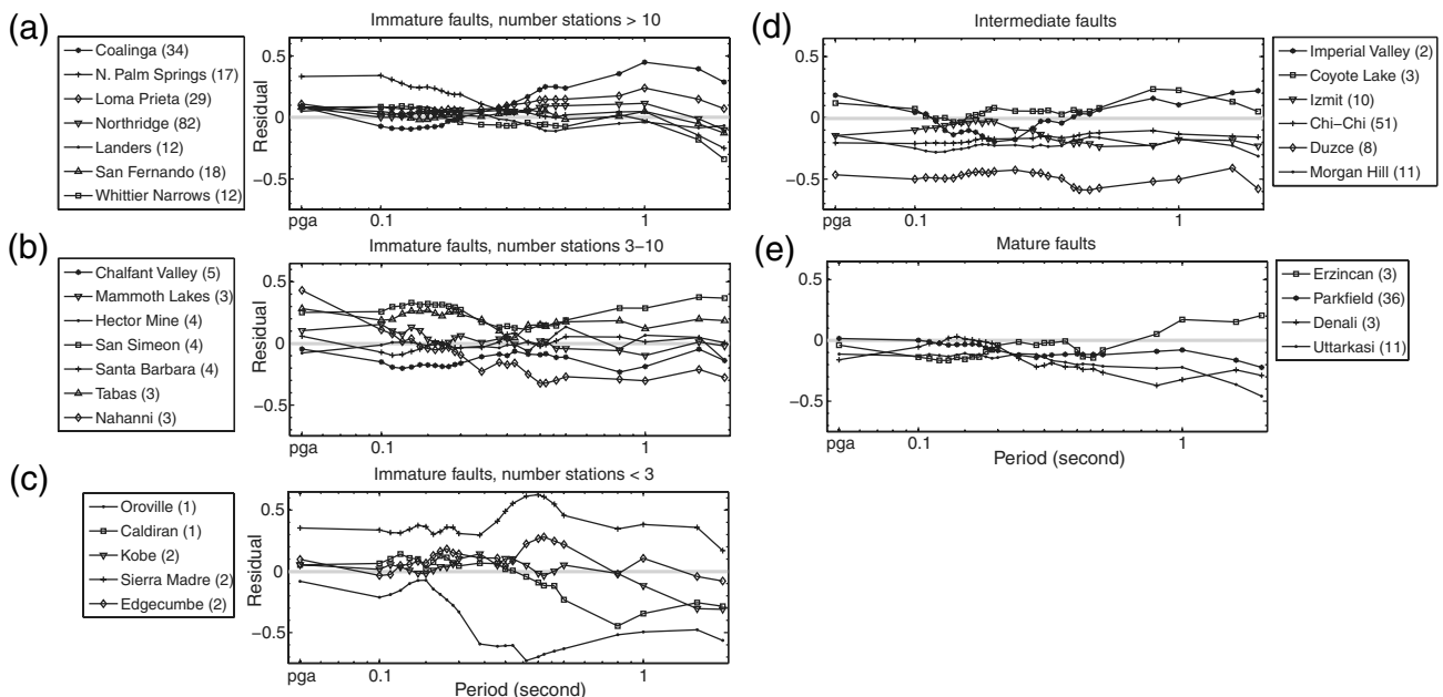
Figure 2. Ratio of response spectral amplitude of individual earthquakes averaged over recording sites to that of the GMPEs of Boore et al. (1997). The zero line represents no bias with respect to the GMPE. The residuals represent the common logarithm of the event/model ratio: +0.1 indicates that the average event ground motion exceeds the model by a factor of 1.26 and -0.1 indicates event ground motion at 0.79 of model value. The number of recording stations for each earthquake is indicated in the legend. (a), (b), and (c) show residuals for earthquakes on immature faults; (d) and (e) show earthquakes on intermediate and mature faults, respectively.
