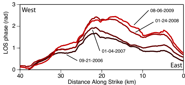
Figure 5.6: Surface creep distribution - Along-strike surface creep rate distribution along the Haiyuan fault at dates 09/21/2006, 01/04/2007, 01/24/2008 and 08/06/2009 for track 240. The zero is indicated by a red square on figure 5.4
