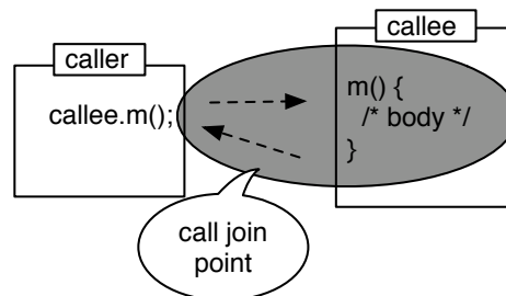
Figure 6.1 – ASPECTJ point-in-region model.
