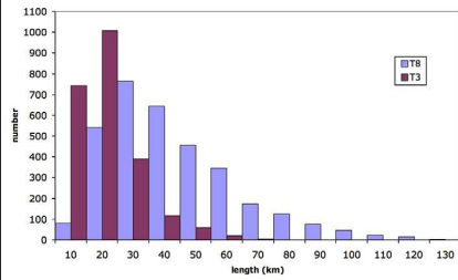
Fig. 7. Dune lengths for the regions of sparse dune field populations (T3) and sand seas (T8). Dunes in the sand seas region are longer than those restricted by sand supply and obstacles.
