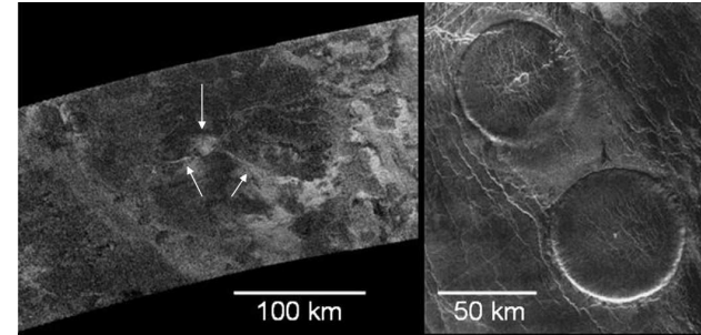
Fig. 3. Titan's Ganesa Macula (left), which we interpret as a cryovolcanic dome or shield, compared with steep-sided ("pancake") domes on Venus imaged by Magellan (NASA press release image PIA00084). Ganesa's central caldera and two channels on the flanks are indicated by arrows. The Magellan image has been rotated (north is to the left) so that the radar illumination is similar to Cassini's (from the bottom of images). See Fig. 4 for the local context for Ganesa.
