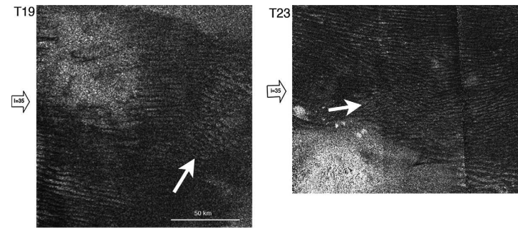
Fig. 8. Dunes from the T19 (October 2006, 10^\circ N, 320^\circ W) and T23 (January 2007, 0^\circ , 350^\circ W) swaths. These regions (located by white arrows) show two dominant dune long axis orientations separated by approximately 60^\circ , indicating a local change in wind pattern. Images \sim 300 m resolution, north is up, arrows indicate direction of radar illumination for each with incidence angle contained.
