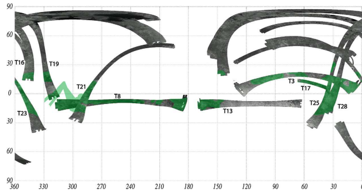
Fig. 4. Plot of dune coverage on Titan as seen in Cassini Radar swaths. All regions on Titan containing a high proportion of dunes as seen in SAR swaths (T1 through T28) are outlined in dark green. Swaths are delineated by flyby number and are labeled close to the major dune areas. Dune-populous areas occur at Titan's equatorial regions.
