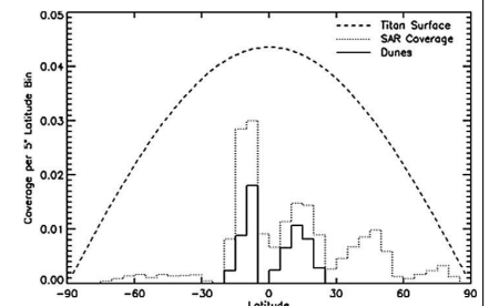
Fig. 11. Distribution of dunes and SAR coverage versus latitude, through the T18 swath. The dashed line indicates complete coverage (equal latitude bins cover smaller areas near the poles). The solid line shows the area covered by dunes, all within 30^\circ of the equator in this plot. The peaks in the SAR coverage (dotted line) are left to right, T7, T8 + T13 covering a large part of Titan just south of the equator, T3 + T17, T4, T16 + T18. SAR passes T19–T30 would increase both overall SAR and dune coverage proportionally at latitudes less than 30^\circ , and would increase the overall SAR coverage to 40–70% at latitudes greater than 60^\circ .
