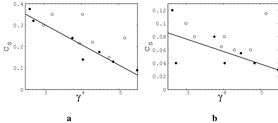
Figure 4.6: L-space. Correlations between the node-degree distribution exponent \gamma and segmentation concentration c_s . Filled circles: scale-free PTN, open circles: PTN with less pronounced power-law decay. Solid lines serve as guides to observe the tendency of c_s to decay with an increase of \gamma . a. Random scenario . Most out of range are the points at c_s = 0.24 , \gamma = (5.16) (Taipei) and at c_s = 0.35 , \gamma = 4.03 (Sydney). b. Recalculated node-degree scenario . Most out of range are the points at c_s = 0.04 , \gamma = 2.72 (Sao Paolo) and at c_s = 0.115 , \gamma = (5.16) (Taipei).
