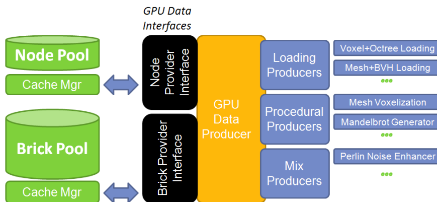
Figure 7.17. Illustration of a GigaVoxels data producer implementing a data provider interface for both the node cache and the brick cache, thus providing both octree nodes and brick data. Multiple kinds of data producers can be used, a few examples are shown here.
