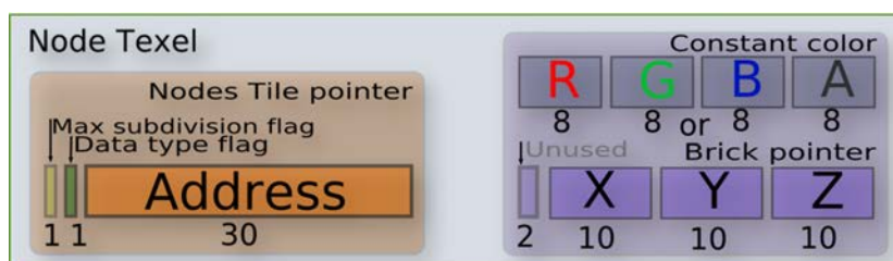
Figure 5.10. Compact octree node encoding into two 32bit values.
