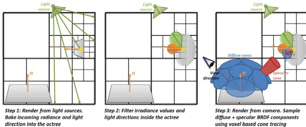
Figure 9.2. Left: Illustration of the three steps of our real-time indirect lighting algorithm. Right: Display of the sparse voxel octree structure storing geometry and direct lighting information.
