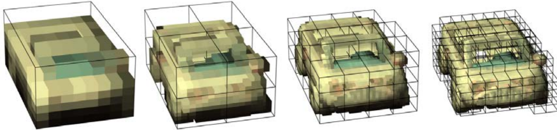
Figure 2.7. Illustration of the brick map structure at multiple resolution used to stored irradiance values for a car model. Source: [CB04a]
