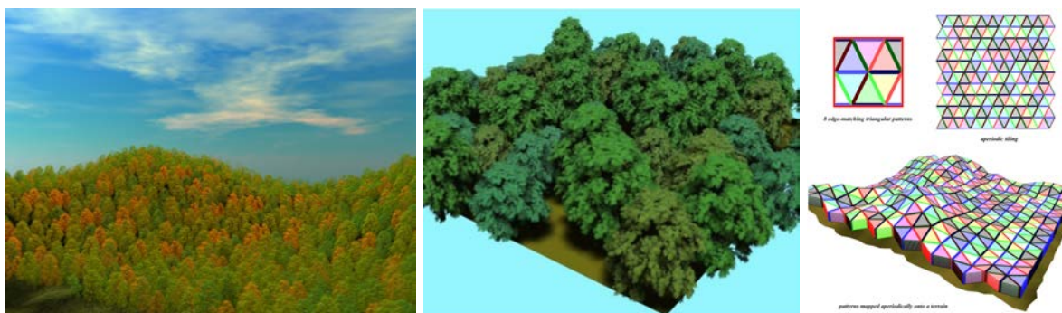
Figure 2.3. Example of forest rendering using volumetric tiles. Source: [DN04]
