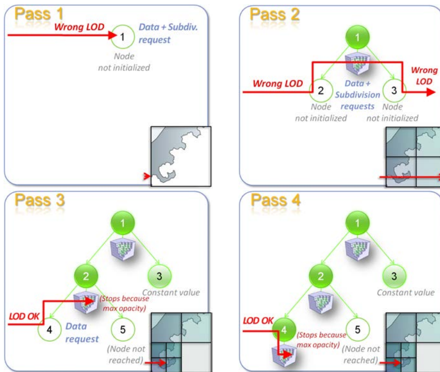
Figure 7.6. Illustration of ray-guided multi-pass update sequence for one ray.
