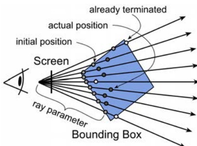
Figure 2.12. Illustration the ray-casting scheme where all viewing rays are processed simultaneously. Source: [RGW + 03]
