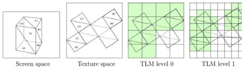
Figure 2.24. The Texture Load Map component of [LDN04] computes the set of visible texture tiles, marked in green, by conservatively rasterizing the geometry in texture space. Source: [LDN04]
