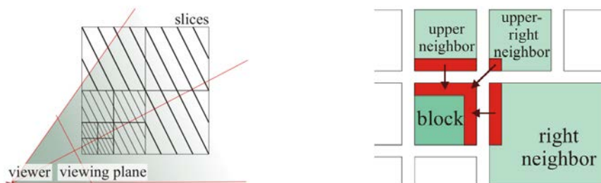
Figure 2.19. Left: Multi-resolution rendering with view-plane aligned slices. Right: Copy of adjacent voxels at different resolution into 3d-texture blocks for correct interpolation. Source: [GWGS02]
