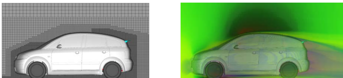
Figure 2.21. An AMR grid used for CFD simulation with refinement around the surface geometry [VSE06].
