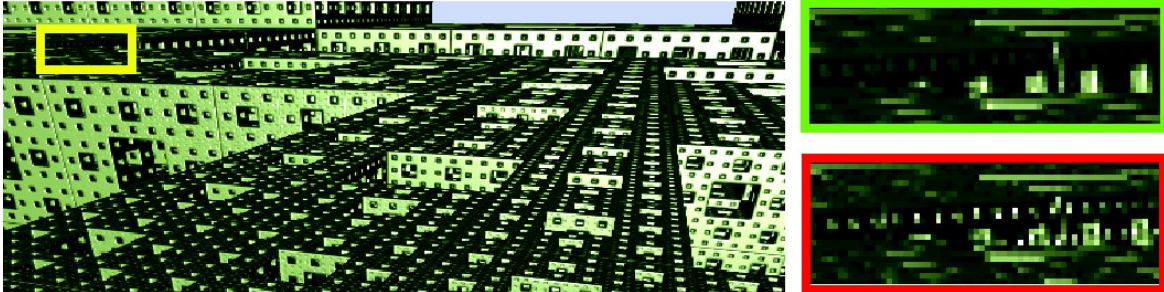
Figure 6.3. Our method (top) based on pre-integrated voxel cone tracing does not show the aliasing artifacts of standard ray-casting with one ray per pixel (bottom).
