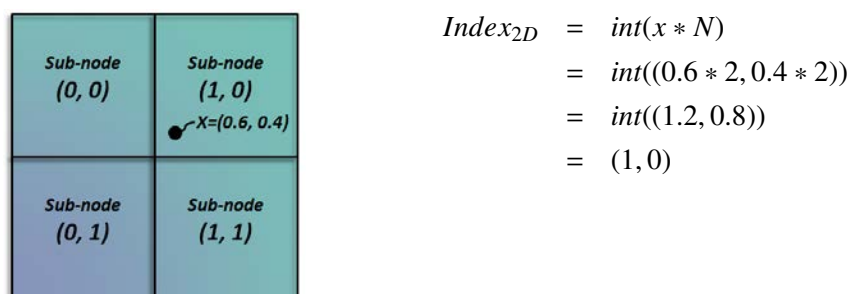
Figure 6.6. 2D localization into a node tile to find the index of the sub-node where x lies.
