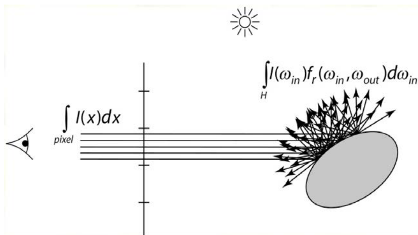
Figure 2.1. Illustration of a 5x per-pixel supersampling used for rendering a shaded sphere. Each direct view-sample integrate indirect lighting following the rendering equation. Source: Don Fussell, University of Texas at Austin, CS384G Computer Graphics course
