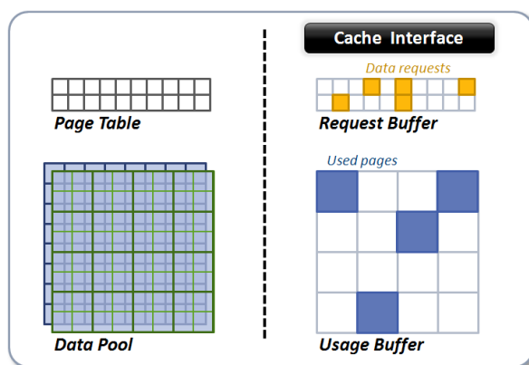
Figure 7.11. Illustration of our cache interface for data requests and tracking of used pages, based on a request buffer and a usage buffer .
