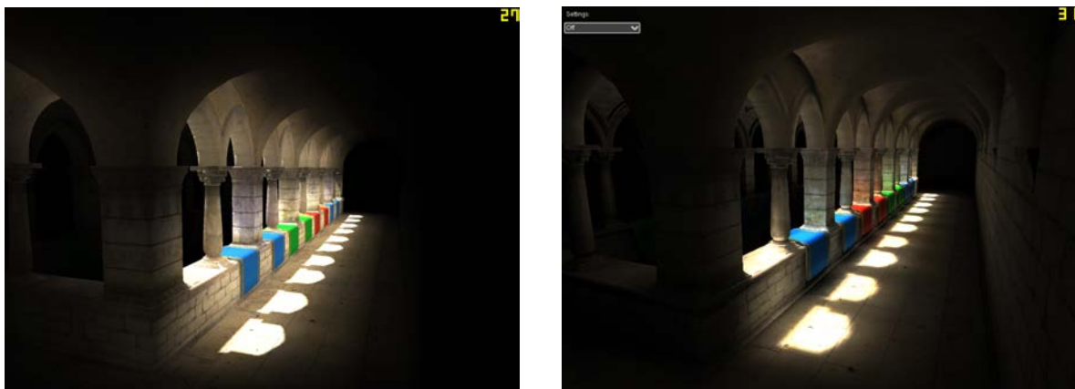
Figure 9.10. Image quality and performance comparison between [KD10] (left, 27FPS) and our approach (right, 31FPS).
