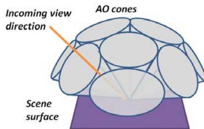
Figure 9.5. Ambient Occlusion is computed via a set of cones launched over the hemisphere associated with a given surface.
