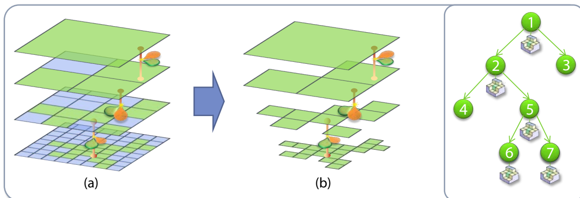
Figure 5.2. Illustration in 2D of our 3D sparse MIP-map pyramid representation, (a) Full MIP-map pyramid, (b) Sparse MIP-map and an illustrative corresponding octree structure.
