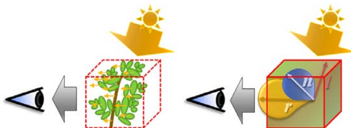
Figure 1.12. Illustration of the pre-filtering of complex geometrical details inside a single voxel element in order to allow the reconstruction of an overall shading contribution.
