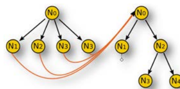
Figure 8.1. Instantiated octree.
