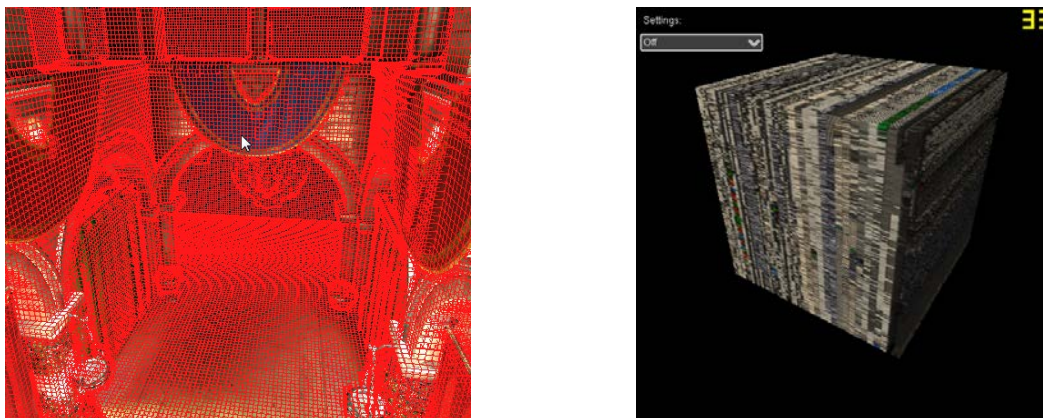
Figure 5.9. Illustration of the packing of non-empty bricks of our sparse voxel octree inside a 3D texture-based brick pool.
