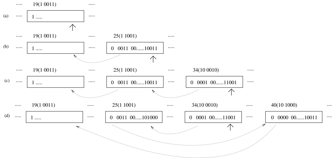
FIG. A.9 – Insertion in a list of occurrences. (a) The list contains only one cell, 19. (b) Insertion of occurrence 25, i = e = 19 . (c) Insertion of occurrence 34 i = 25, e = 19 and l = 25 . (d) Insertion of occurrence 40 i = 34, e = 19, l = 25 , 19 is already coded in the cells 34 and 25, 40 is added after 25.
