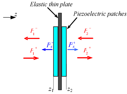
Fig.3-1 The active plate
