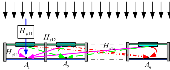
Fig.6-2 The transfer function schematic of multi-cell hybrid structure
