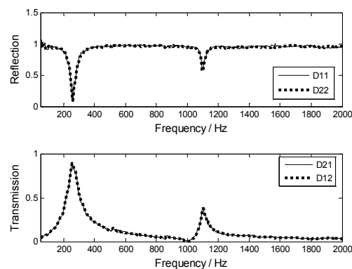
Fig.5-6 The reflection and transmission coefficients of the radiating plate
