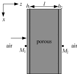
Fig.2-10The total transfer matrix of the plate/porous material/plate
