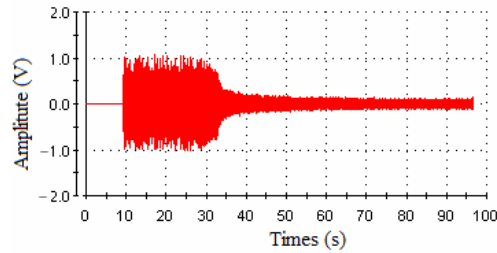
Fig.5-13 The error sensor signals before and after active control
