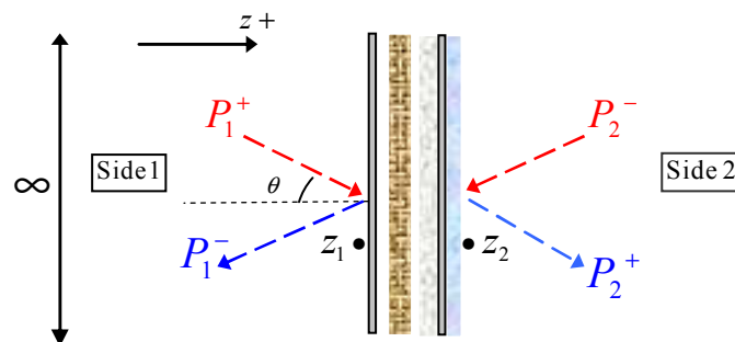
Fig.2-2 The schematic of a passive system with infinite lateral dimensions
