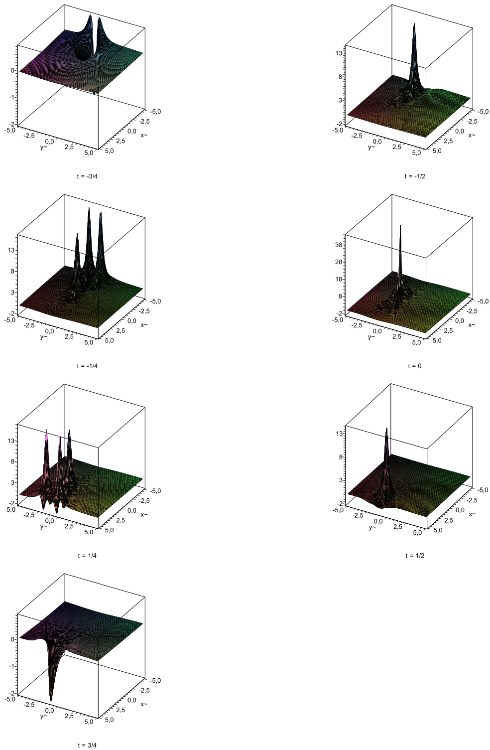
Figure 10: Solution of KP-I with \varphi_4 = \frac{5+\sqrt{5}}{96} \sqrt{10 - 2\sqrt{5}}
