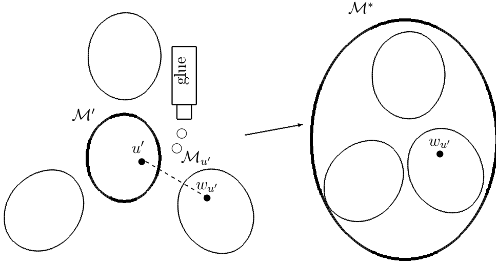
Figure 7.5: Gluing the super-additive-models \mathcal{M}'_u in order to get \mathcal{M}^*
