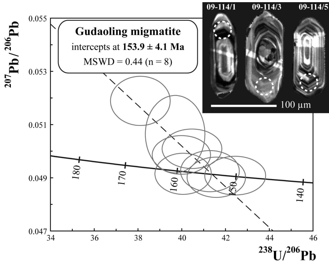
Figure 4.23: Tera and Wasserburg (1972) Concordia diagram for 09-114 sample. Examples of CL images of zircon are shown with location of analytical points. The diameter of ablation pit is ca. 30\ \mu\text{m} . Data-point error ellipses are plotted as 2\sigma .
