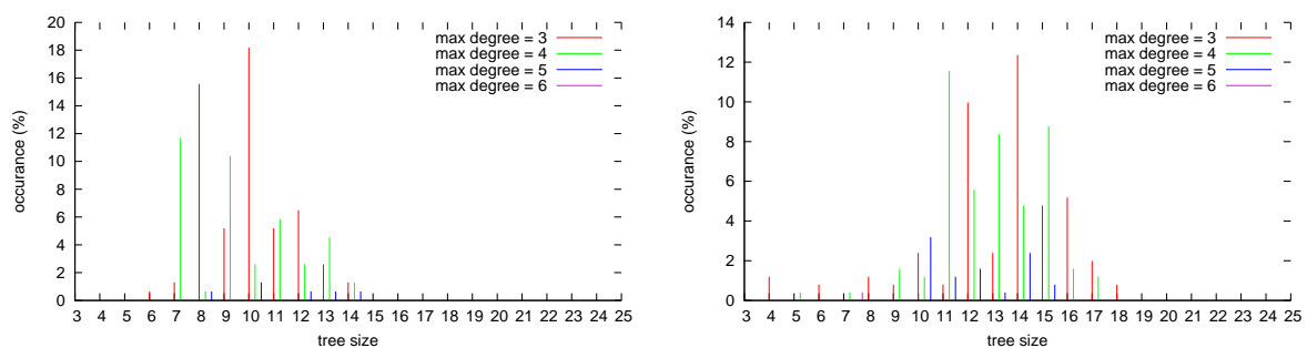
FIGURE 11.9: Distributions for a grid sided by 80. Left: dancer data set. Right: hand data set.
