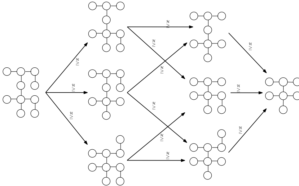
FIGURE 10.1: Example of asymmetric homeomorphic relations on a set of homeomorphic trees.
