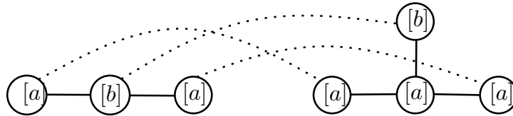
FIGURE 8.8: An invalidate constrained mapping: the center relationship preservation condition is not respected.
