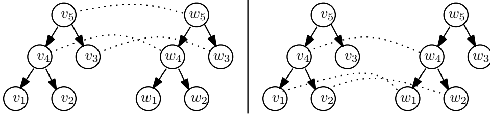
FIGURE 8.10: At left: a mapping which is top down. At right: a mapping which is not top down.
