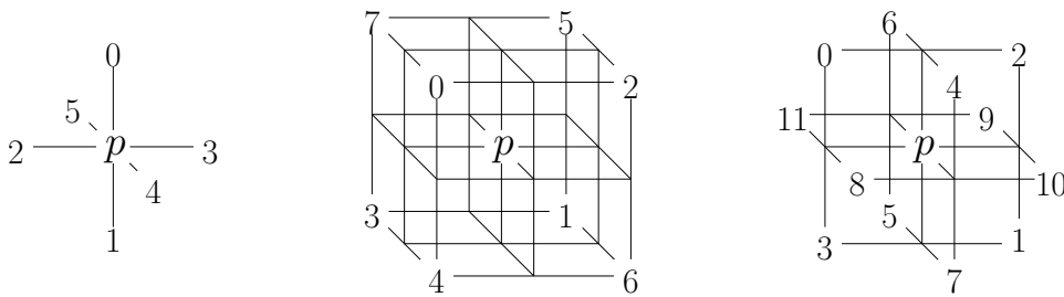
FIGURE 4.9: From the left to the right: Directions used for directional thinning algorithms with 6, 8 and 12 sub-iterations. Each number i represents a voxel which have to be out of the object to allow the deletion of p in the i th sub iteration.
