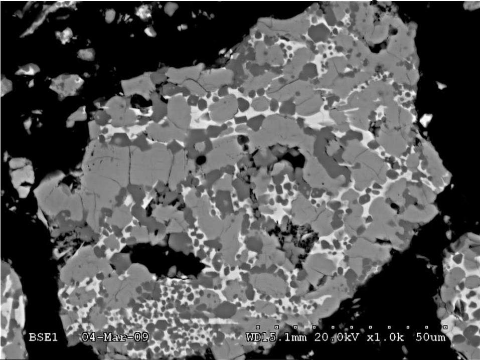
Figure 2A5-3: Typical FEG-SEM BSE image of clinker k165
