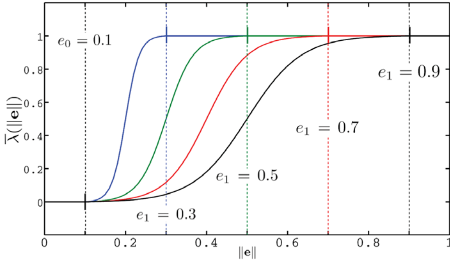
Figure 6.1 – Switching function \bar{\lambda}(\|e\|) .
