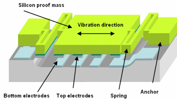
Fig. 2.14 Proposed energy harvester design: Proof mass Configuration (PC)
