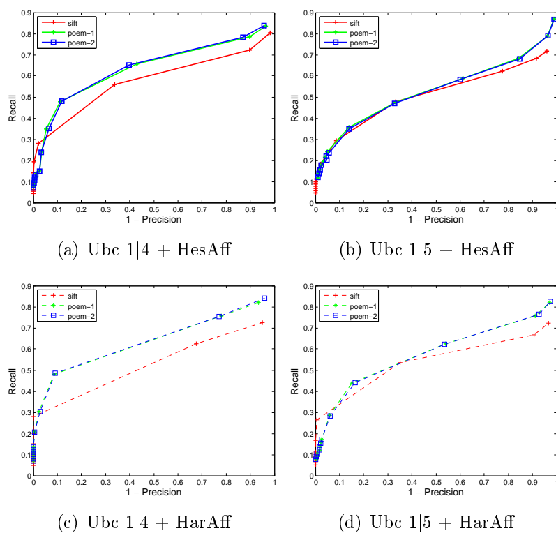
Figure 7.5 – Robustness to compression artifacts.
