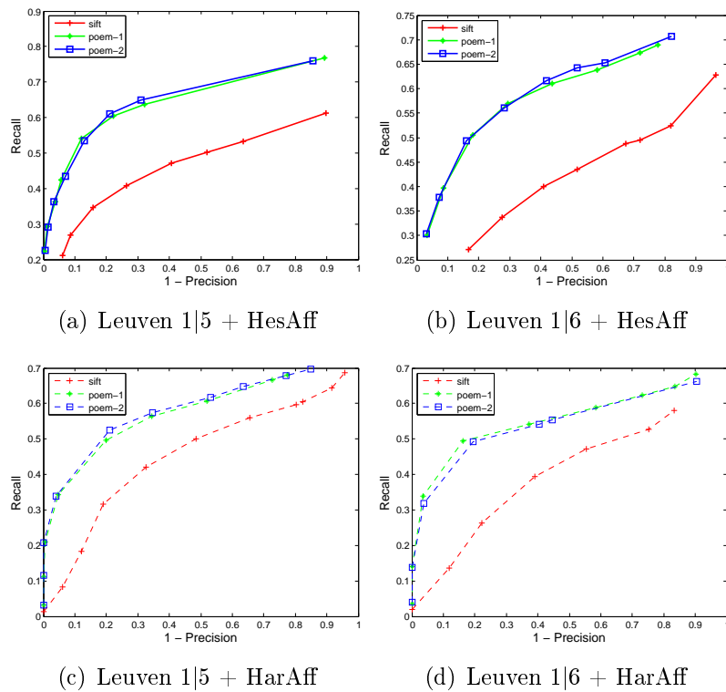
Figure 7.4 – Robustness to lighting changes.
