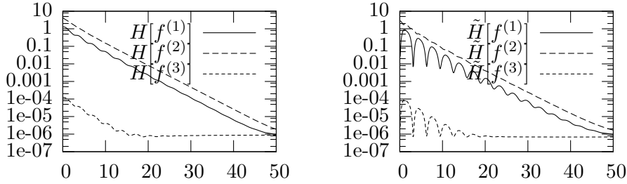
Figure 7: 1D Vlasov with confining potential. From this comparison, it is quite clear that the oscillation rate is the same for both initial functions, even if the behaviour is different.
