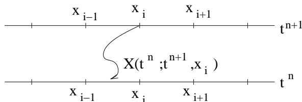
Figure 1: The direct Semi Lagrangian reconstruction, based on following backward the characteristics.
