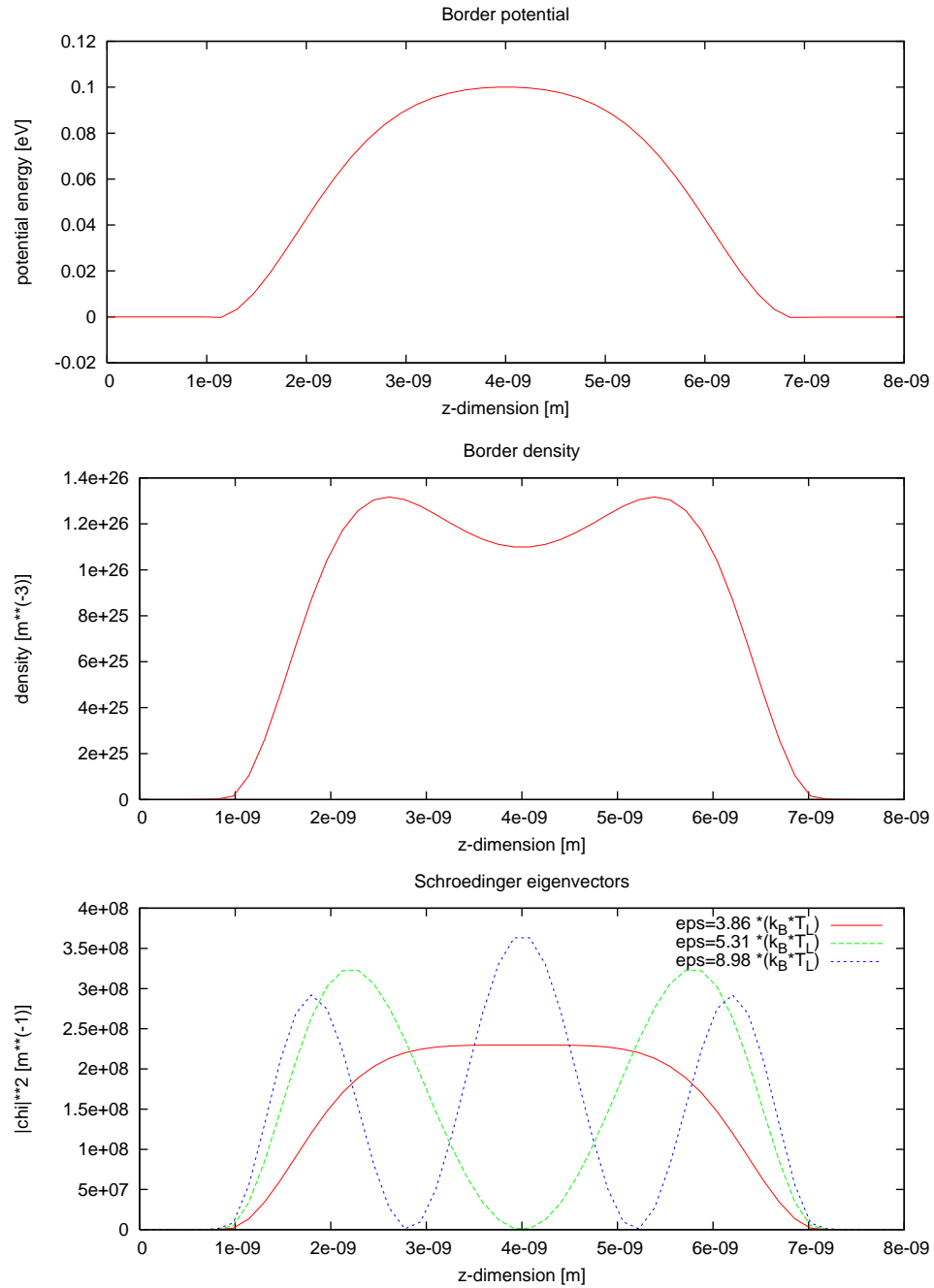
Figure 4: Border potential. The grid is 64 points along the z -dimension. Top: the potential energy at contacts. Center: the free electron density at contacts. Bottom: the Schrödinger eigenfunctions corresponding to the three first energy levels.
