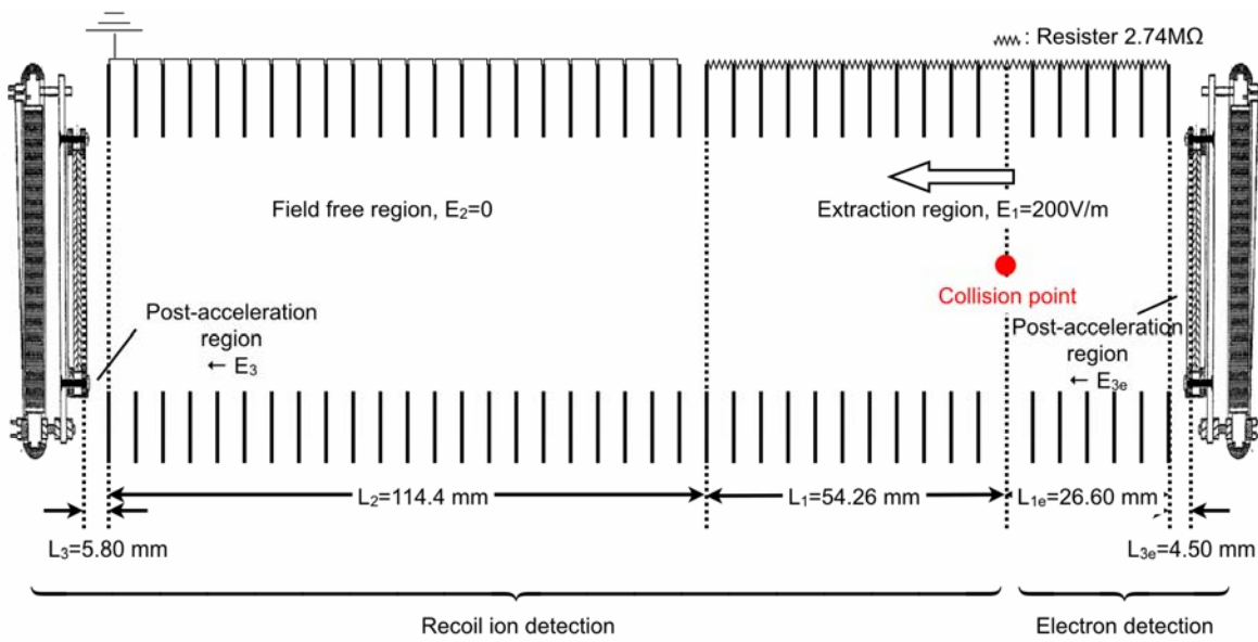
Figure II- 13 Spectrometer for NO 2 : Wiley-MacLaren time focusing condition
