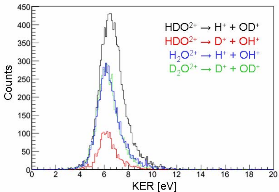
Figure V- 16 KER distributions of four dication two-body dissociation channels induced by 170keV \text{Ne}^{10+} , without normalization.
