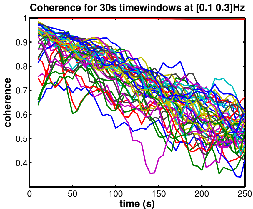
FIG. 8.6 – Coherence versus lapse-time for a 30 second sliding window in the coda. Results shown for 98 station pairs, for correlation functions are bandpassed at [0.1 0.3]Hz.
