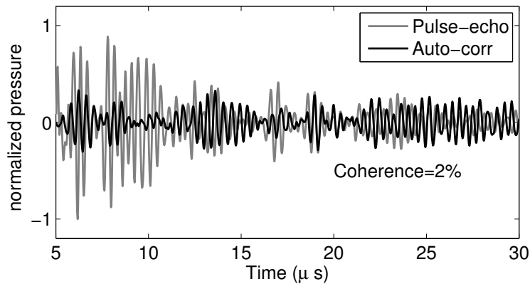
FIG. 5.8 – Comparison of the pulse-echo data h(R, R, t) obtained in the active experiment and the average autocorrelation \partial_t h(S, R, t) \times h(S, R, t) .
