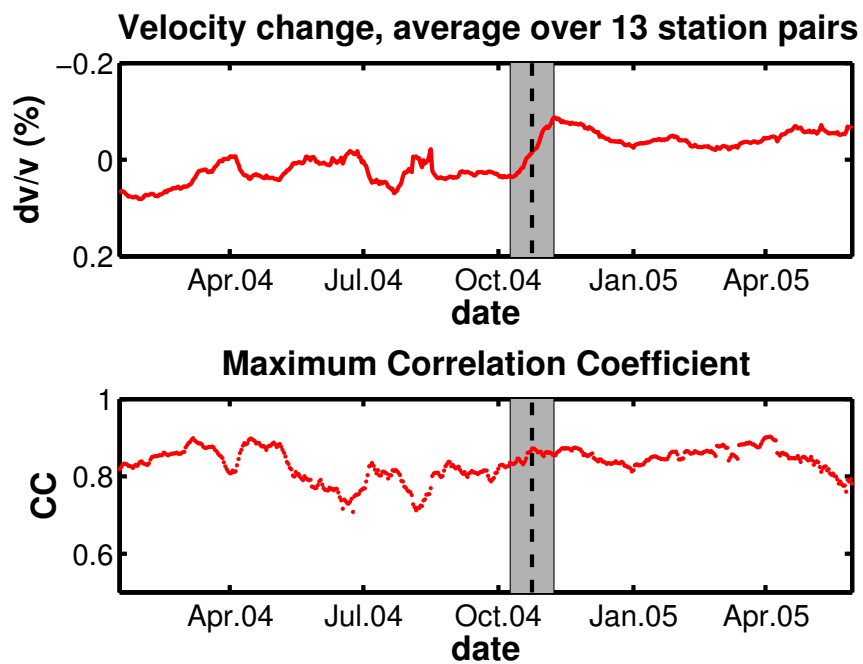
FIG. 8.9 – Top : dV/V measurements averaged over 13 station pairs. Bottom : corresponding maximum correlation coefficient ( CC ). Correlation functions are band-passed for [0.1\ 0.3] Hz. The black dashed line indicates the date of the M_w = 6.9 Chuetsu event. The grey area indicates the extent of the 30-day stack.
