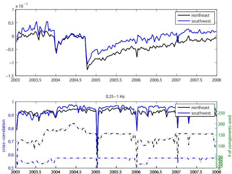
FIG. 10.1 – Relative velocity change measured near Parkfield, using the whole 9-component Green's tensor. Correlation functions are bandpassed at [0.25 \text{--} 1] \text{ Hz} , and averaged using a 20-day sliding window. The reference function used is the average of 3 months of noise around July, 2004. (Courtesy Ozgun Konca.)
