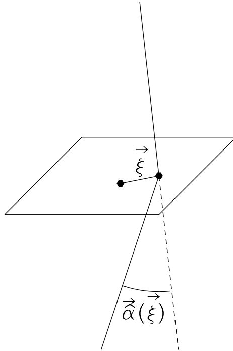
Figure 3.1: A light ray intersecting the lens plane at \xi is deflected by an angle \vec{\alpha}(\xi) . Credit: Narayan & Bartelmann (1996)
