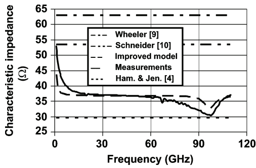
Fig. 8. Simulated and measured characteristic impedance of a 65-nm technology microstrip line.
