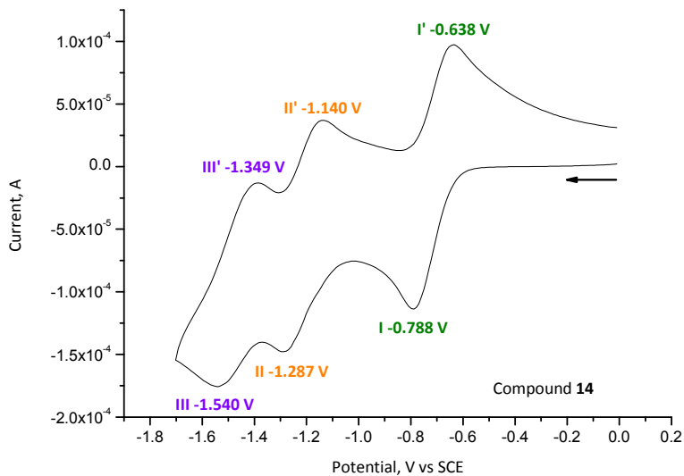
Figure 58. Cyclic voltammogram of compound 14 at silicon electrode. [\mathbf{14}] = 1 \times 10^{-3} M in acetonitrile with 10^{-1} M \text{Bu}_4\text{NBF}_4 as supporting electrolyte. Scanning rate: 100 mV/s.
