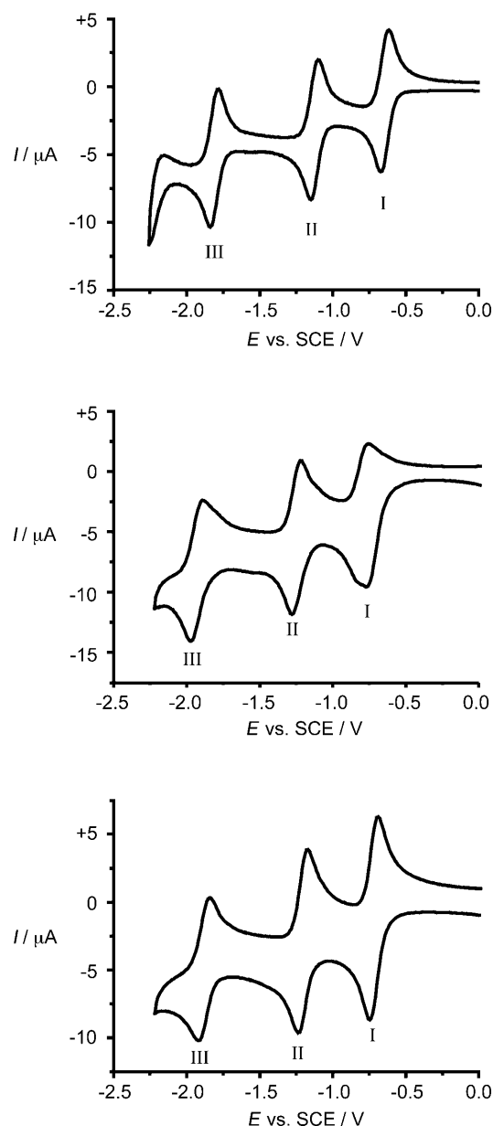
Figure 6. Cyclic voltammograms of (NBu_4)_3[PW_9O_{34}(tBuSiOH)_3] (top), (NBu_4)_3[PW_9O_{34}(tBuSiO)_3Ge(CH_2)_2CO_2H] ( 1 ) (middle), and (NBu_4)_3[PW_9O_{34}(tBuSiO)_3Ge(CH_2)_2CONHCH_2C\equiv CH] ( 2 ) (bottom) at a glassy carbon electrode. ( [POM]=1\times 10^{-3} mol L –1 in acetonitrile, 0.1 mol L –1 NBu_4BF_4 , 20 mV s –1 ).
