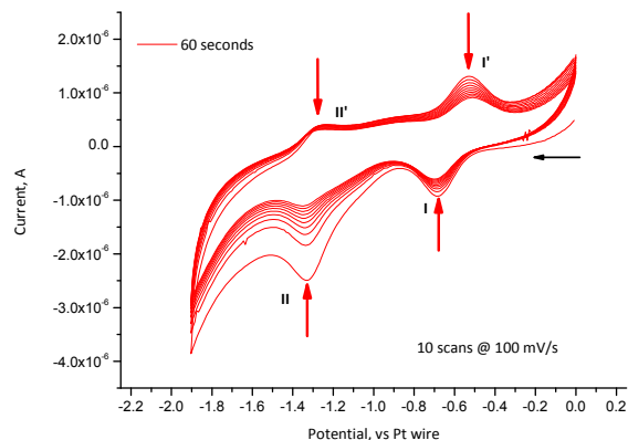
Figure 45. Stability test of the substrate Si-FE17 towards cycling in propylene carbonate (1.0 M Bu 4 NPF 6 ).
