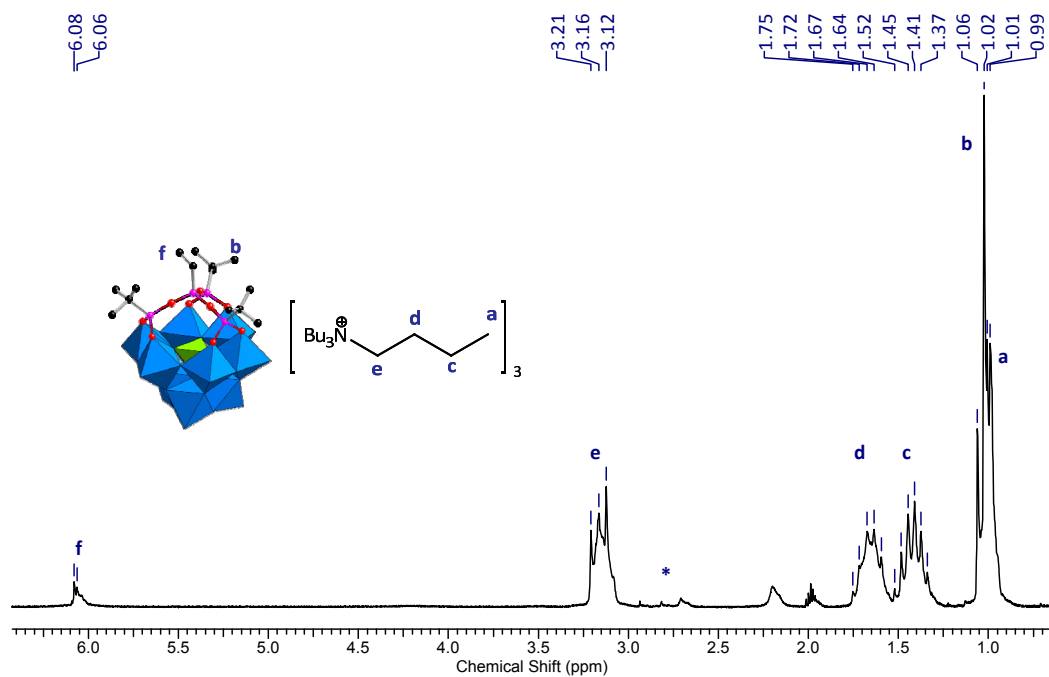
Figure 11. The 1 H NMR (200.13 MHz, CD 3 CN) spectrum of compound 5 (* = DMF).
