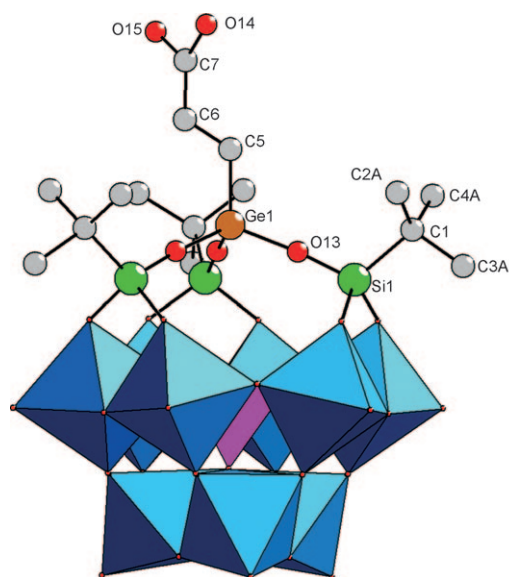
Figure 5. Mixed polyhedral and ball-and-stick representation of [PW_9O_{34}-(tBuSiO)_3Ge(CH_2)_2CO_2H]^{3-} ( 1a ).
