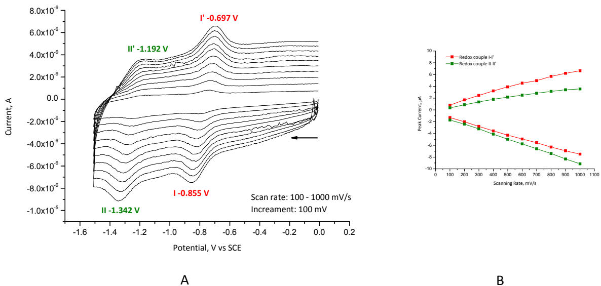
Figure 51. (A) Cyclic voltammetric curves of substrate GC-FS17 at different scan rates in acetonitrile (0.1 M \text{Bu}_4\text{NBF}_4 ). The GC-FS17 substrate was formed by spontaneous electrografting for 60 minutes. (B) Linear dependence of peak current on scan rate. Electrode surface: 0.07 \text{ cm}^2 area.
