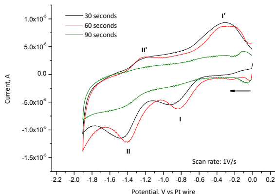
Figure 44. Overlaid CV of substrate Si-FE17 in propylene carbonate (1.0 M Bu 4 NPF 6 ), at an imposed potential of -1.7 V vs Pt wire for 30, 60 and 90 seconds, respectively.
