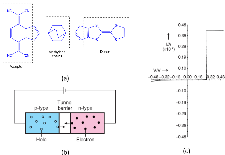
Figure 3. Explanation of molecular rectifier: (a) model molecule proposed by Aviram and Ratner, (b) p - n junction, and (c) calculated I - V characteristics. 3
