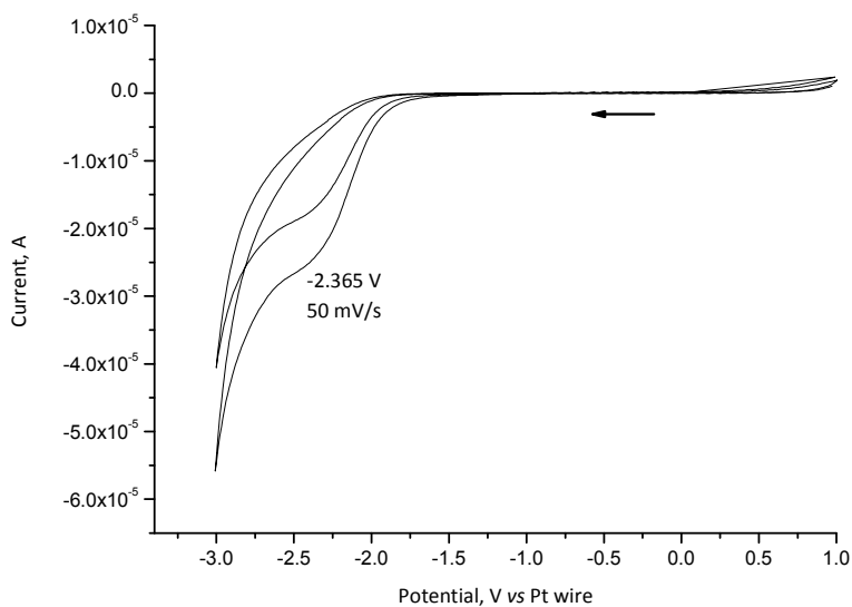
Figure 8. Cyclic voltammetry recorded for Si-A15 (ionic liquid). Scan rate: 50 \text{ mV}\cdot\text{s}^{-1} . Conditions: neat/ 180^\circ\text{C}/2\text{hrs} . Electrode surface: 0.75 \text{ cm}^2 exposing 0.55 \text{ cm}^2 area.
