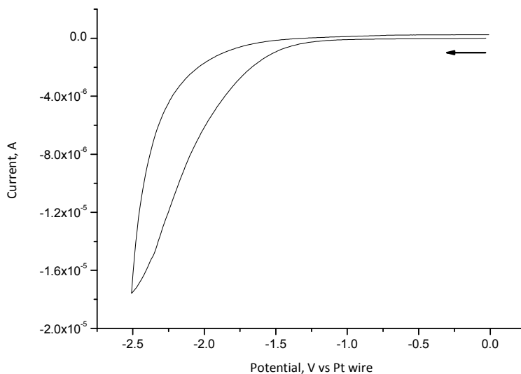
Figure 21. Cyclic voltammetry recorded for Si-C14 ( 10^{-1} M \text{Bu}_4\text{NBF}_4 in acetonitrile). Scan rate: 20 \text{ mV}\cdot\text{s}^{-1} . Electrode surface: 0.75 \text{ cm}^2 exposing 0.55 \text{ cm}^2 area.
