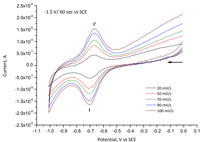
Figure 46. (A) Cyclic voltammograms of substrate Si-FE17 at different scan rates in propylene carbonate (1.0 M Bu 4 NPF 6 ). The Si-FE17 substrate was formed by potentiostatic electrografting at -1.5 V vs SCE for 60 seconds in acetonitrile (0.1 M Bu 4 NBF 4 ). (B) Linear dependence of peak current on scan rate. Electrode surface: 0.60 cm 2 exposing 0.36 cm 2 area.
