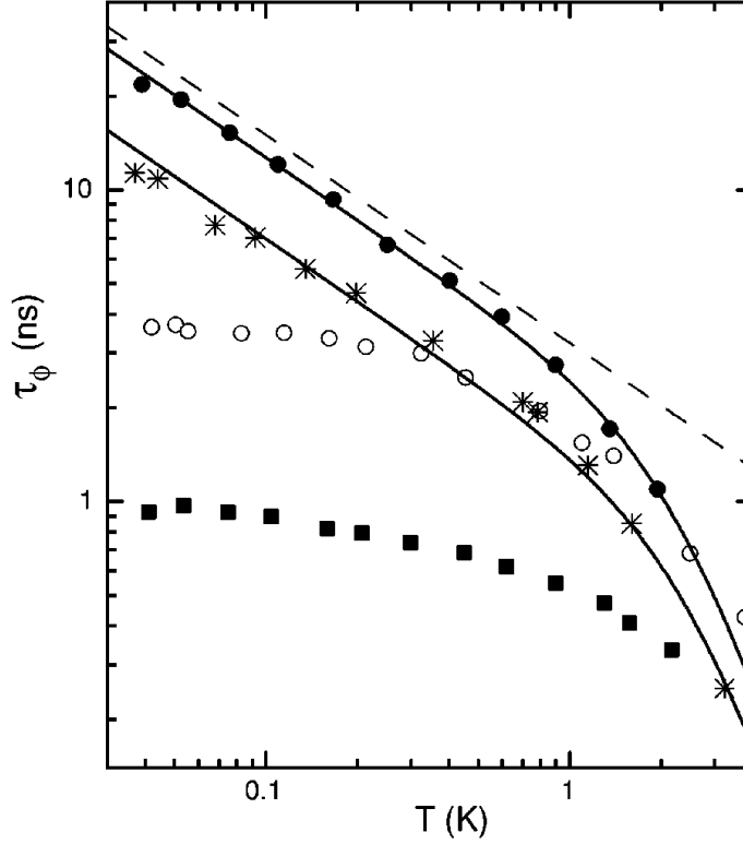
Figure 2.7: Behavior of the phase coherence time \tau_\phi for different metallic wires (silver for dots, gold for stars and copper for squares) via magnetoresistance measurements. In the purest samples (solid circles and stars) we observe a dependence \tau_\phi^{-1}(T) = AT^{2/3} + BT^3 (plain lines). Dashed line represents the contribution with power 2/3 for silver. We attribute down to 0.1K the decoherence to electron-phonon and electron-electron interactions. For samples with more impurities deviations with the power law is observed. Saturation at very low temperature has been attributed to other dephasing mechanisms. Extracted from [75].
