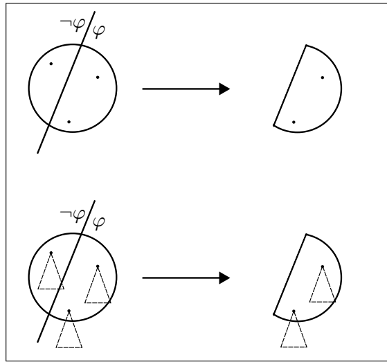
Figure 4.3: AGM expansion by \phi ( above ) and BMS update by a private announcement of \phi ( below )
