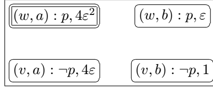
Figure 5.7: Situation after she believed that her colleague's lecture is on Thursday ( \neg p ) and she heard him saying that he would come on Thursday ( b ).
