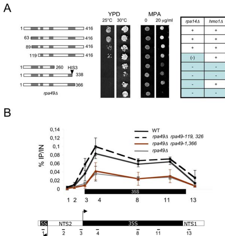
Figure 4. Mutagenesis of RPA49. (A) Growth defects of rpa49 mutants. Strain D704-7C ( rpa49Δ ) was transformed with pVV200 plasmids (Van Mullem et al., 2003) bearing the relevant wild-type and rpa49 mutants corresponding to progressive N- and C-terminal
