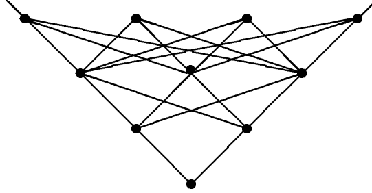
FIGURE 3.1. Arbitrary Large Antichains
