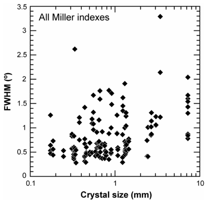
Figure 3-4. Full width at half maximum (FWHM) versus crystal size (chosen to be the diameter of circle of equivalent area to an ellipsoid fitted to outline), for all hkl indexes at a time.
