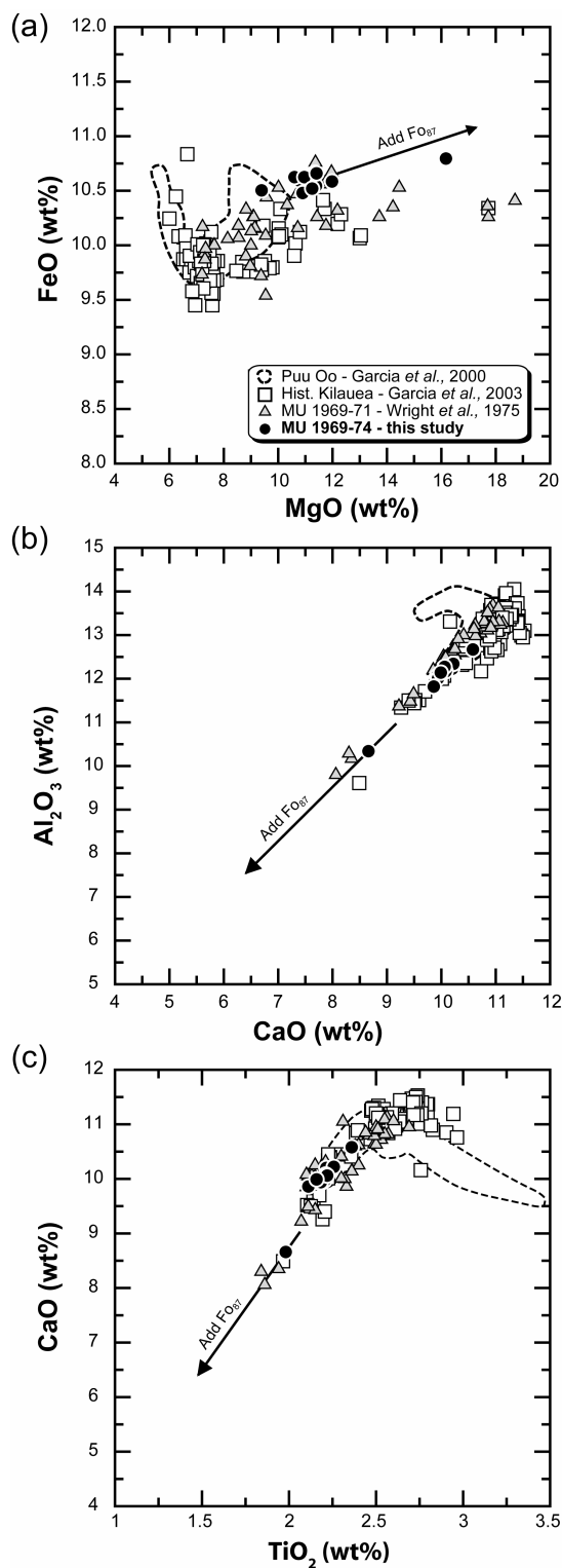
Figure 1-4. Selected major-oxide variation diagrams illustrating the compositional tendency that can result from addition of olivine Fo_{87} to the whole-rock composition: (a) MgO vs FeO, (b) CaO vs Al_2O_3 and (c) TiO_2 vs CaO. Notice that the MU lavas, along with other Kilauea lavas, are clearly olivine-controlled.
