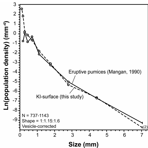
Figure 2-13. Comparison of our mean surface CSD versus recalculated pumice CSD from data of Mangan (1990). Number in parentheses at the right end of the KI-surface CSD refers to the number of grains analysed in the last CSD bin (largest crystal sizes).
