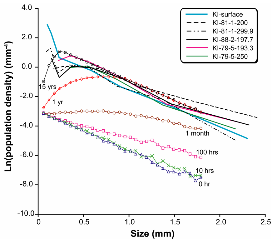
Figure 2-15. Modeled CSDs after olivine settling. Some lake CSDs at depths around 60 m and greater have also been plotted for scale and result validation. The initial CSD was taken to be the straight middle segment of our mean surface CSD, at size range 0.5-3.0 mm. The model used here follows the procedure of Higgins (2002b).
