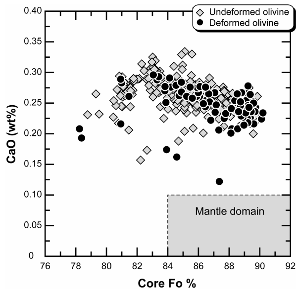
Figure 1-8. CaO content versus Fo content (%) of the core of both the undeformed and deformed olivine crystals analyzed in the Mauna Ulu lavas of this study. All olivines plot above the mantle domain indicated as the shaded area. Mantle domain after Kamenetsky et al. (2006), Simkin & Smith (1970) and Thompson & Gibson (2000).
