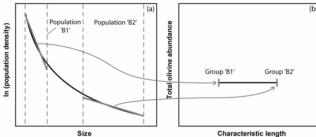
Figure 1-13. Schematic diagrams illustrating the segmentation of CSDs. (a) The original CSD curve is in black. The segments in grey both at the left and right sides of the CSD are for the olivine populations B1 and B2, respectively. Each segment (straight line) represents a mean of several CSD bins. (b) A plot of total sample olivine abundance vs. characteristic length for the two segments. The calculation inferred from the CSD segmentation permits placement of two points for the same sample of a given olivine abundance, representing here by the two small vertical bars in grey. The left bar corresponds to the population B1 segment and the right bar to the population B2 segment. The length of the horizontal line that links the vertical bars gives us information on the degree of curvature of the CSD, and thus on the level of mixing of at least two different crystal populations, for example.
