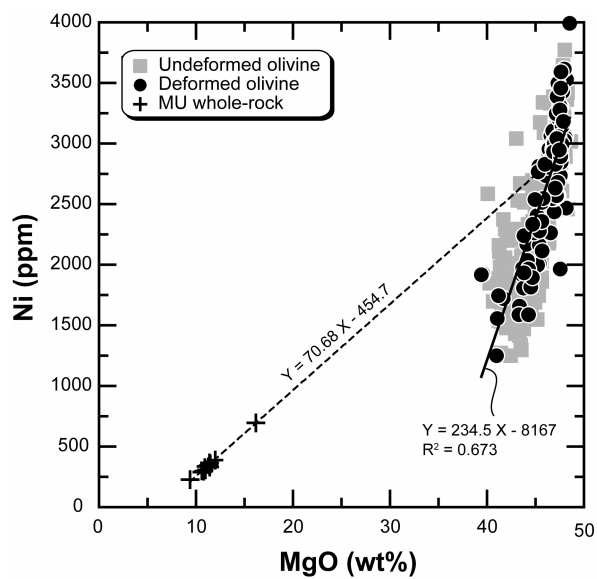
Figure 1-19. Plot of Ni versus MgO for Mauna Ulu (MU) lavas and both undeformed and deformed olivines. Linear regression lines along with their equation are shown for both whole-rock analyses (dashed line) and deformed olivine in the lavas (simple line). The intersection of those two regression lines yields the composition of the added olivine.
