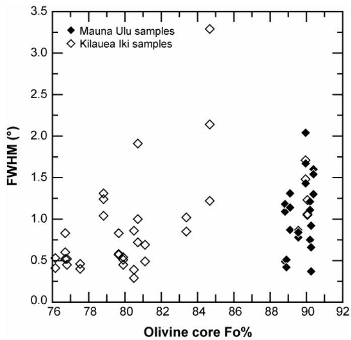
Figure 3-3. Full width at half maximum (FWHM) versus olivine core forsterite (Fo) content for all samples analysed by \mu XRD.
