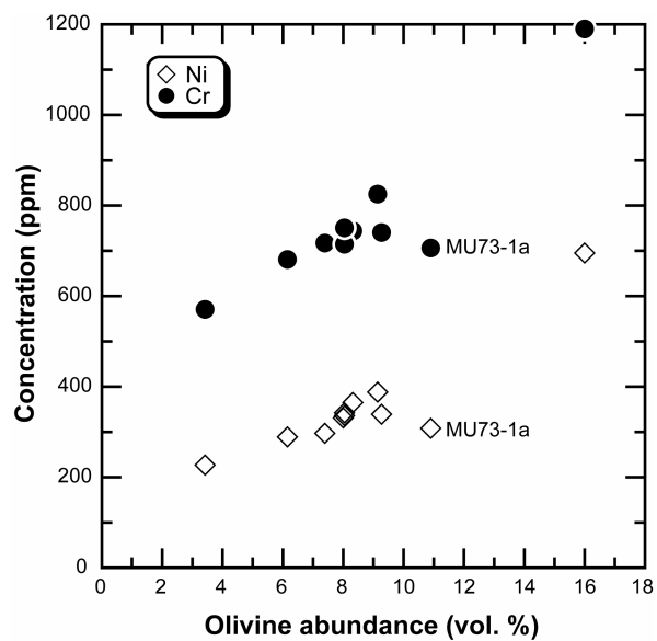
Figure 1-6. Ni and Cr whole-rock content versus olivine abundance for the Mauna Ulu lavas.
