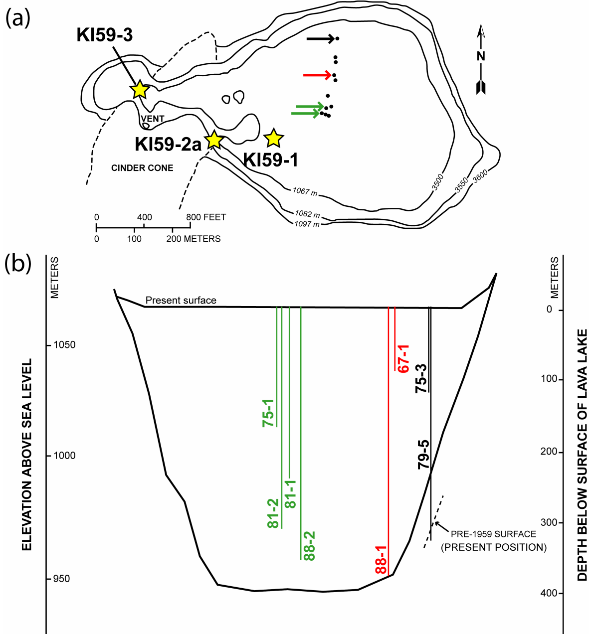
Figure 2-1. a) Plan view of the post-1959 surface of Kilauea Iki (modified after Helz, 1993). The larger dots indicate locations of holes drilled from 1967-1988. b) N-S cross-section of Kilauea Iki lava lake, with projected drill holes shown. Vertical exaggeration is 4:1. Modified after Barth et al. (1994).
