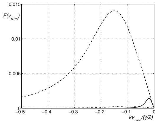
FIG. 7. Effective force \bar{F}(v_{\text{rms}}) in units of \hbar k \gamma versus kv_{\text{rms}}/(\gamma/2) for \text{Ca}^+ wavelength ( \lambda_w=732 nm and \lambda_{st}=866 nm) and \gamma/2\pi=20 MHz, \beta_{eg}=1 . The different curves are for different values of \Omega_w/2\pi : 0.1 MHz (solid line and dotted-dashed line) and 1 MHz (dashed line). \Delta_{st} is fixed to -10\gamma and \Omega_{st} is chosen to obtain the maximum signal, according to Eq. (10), only for the curves plotted with the solid line and the dashed line, \Omega_{st}=34 MHz (solid line), 106 MHz (dashed and dotted-dashed line), \Delta_w=\delta_{LS}-\Gamma_{\text{eff}}/2 .
