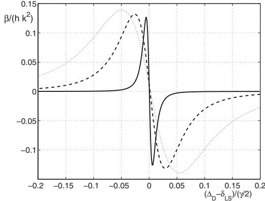
FIG. 5. Damping factor \beta in units of \hbar k^2 versus the relative detuning of the weak transition from the light shift. \text{Ca}^+ wavelengths are used ( \lambda_w=732 nm and \lambda_{st}=866 nm) and \gamma/2\pi=20 MHz. The three curves are for different values of \Omega_w/2\pi : 0.1 MHz (solid line), 0.5 MHz (dashed line), and 1 MHz (dotted line), \Delta_{st}/2\pi is fixed to -10\gamma and \Omega_{st} is chosen to obtain the maximum signal, according to Eq. (10).
