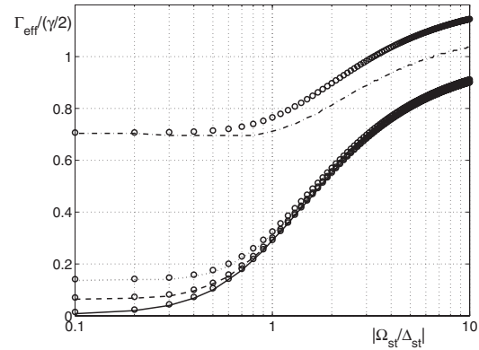
FIG. 4. FWHM of the resonance curve of \phi_e with \Delta_w , in units of \gamma/2 , as a function of the ratio |\Omega_{st}/\Delta_{st}| , for a system identical to Fig. 3. \Delta_{st}/2\pi = -200 MHz and \Omega_{st} varies from 0.1|\Delta_{st}| to 10|\Delta_{st}| . The different curves are for different values of \Omega_w which are 0.1 MHz (solid line), 0.5 MHz (dashed line), 1 MHz (dotted line), and 5 MHz (dotted-dashed line). The lines give the numerical results from the master equation, with no approximations. The symbols plot the FWHM as given by Eq. (15).
