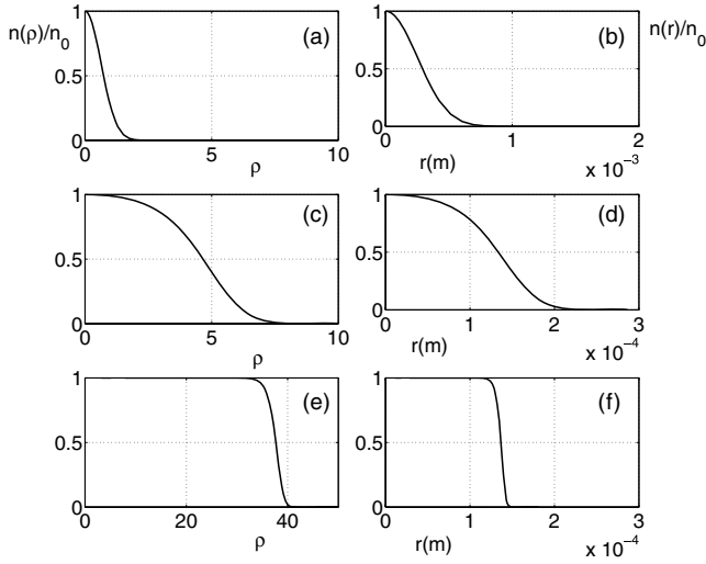
Figure 2. Density profiles versus the reduced radius \rho ( a , c , e ) or the radius r ( b , d , f ) for a prolate cloud with 10^5 ions per mm, at different temperatures ( a , b : T = 10\,000 K, \gamma = 5 , c , d : T = 300 K, \gamma = 0.04 , e , f : T = 5 K, \gamma = 10^{-15} ). The scaling factor \lambda_D between \rho and r is calculated for \text{Ca}^+ ions in a trap with \omega_x/2\pi = 1 MHz. Note that the x -axis of figure b has a different scale from d and f , and that the x -axis of figure e has a different scale from a and c .
