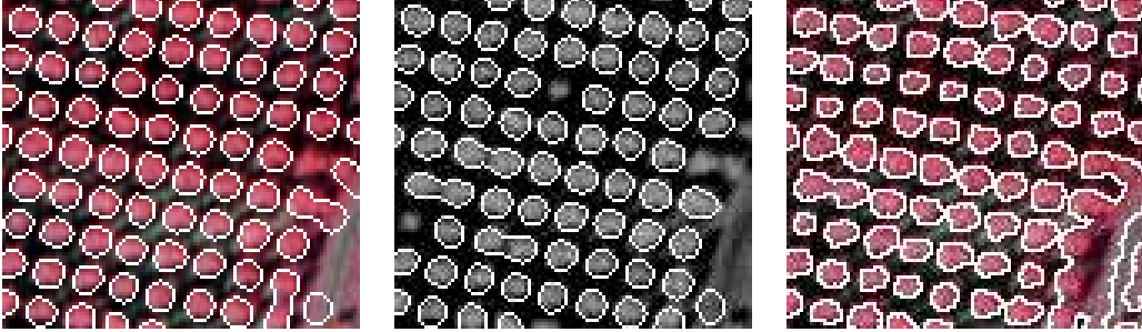
Figure 4.30: Results obtained on the image shown in figure 4.7 middle, using the CAGOC model (left) (17.5, 3.58, 2.5), the AGOC model (middle) (0.2, 3.58, 2.5), and the classical active contour model (right). © IFN
