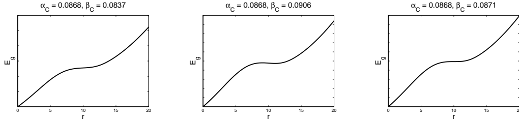
Figure 3.7: Graphs of the energy of a circle.
