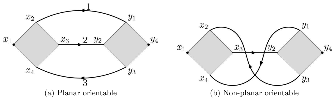
Figure 4.5: Graphs in the Moyal space
