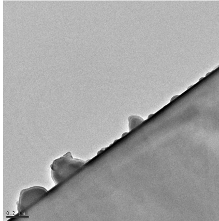
Fig. (7-7): Image of the section of crystallite grown on the reactive interface (11\bar{2}0)_{ZnO} \parallel (1\bar{1}02)_{sapphire} and used for the ED measurements. The small black line in the left side, on the bottom, is the scale and is 0.2 \mu\text{m} .
