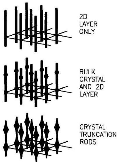
Fig (6-2): Schematic diffraction patterns corresponding to Fig (6-1). (a) for the isolated monolayer, (b) for the surface a 3D crystal, (c) more realistic representation showing variation of intensity along crystal truncation rods (CTRs)
