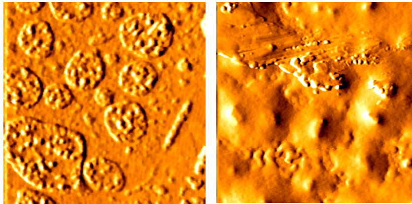
Fig. (7-5): Details of some of the AFM photos of the interface reported in Fig. (7.4). The left image is a section 3 \times 3 \mu\text{m} of the sample heated at 800 °C for 20 minutes, while the right one is a section 5 \times 5 \mu\text{m} of the sample heated at 800 °C for 40 minutes.
