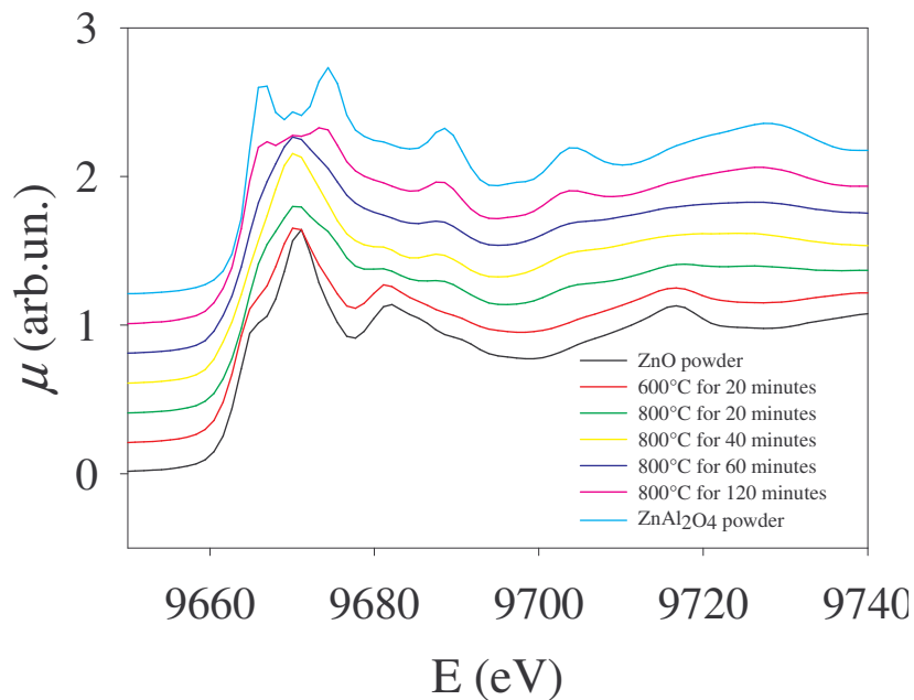
Fig. (4-5): XANES manifold for the reactive interface A changes from increasing heating temperature and time at 800 °C. For comparison purposes the spectra of powder ZnO and ZnAl 2 O 4 are reported.
