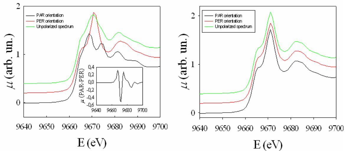
Fig. (3-3): Zn-K edge XANES. The left figure refers to the reactive interfaces (0001)_{ZnO} \parallel (11\bar{2}0)_{sapphire} and (0001)_{ZnO} \parallel (0001)_{sapphire} where a huge linear dichroic effect is very well visible. The right figure refers to the reactive interface (11\bar{2}0)_{ZnO} \parallel (1\bar{1}02)_{sapphire} where no linear dichroic is found. For comparison purposes the unpolarized spectra are reported.
