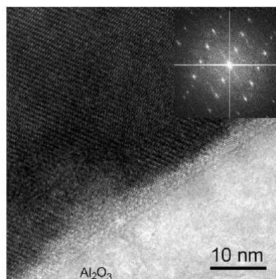
Fig. (7-7): HRTEM image for the (11\bar{2}0)_{ZnO} \parallel (1\bar{1}02)_{sapphire} interface at 800 \text{ }^\circ\text{C} for 120 minutes. The inset shows an electron diffraction pattern of the reaction product
