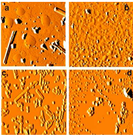
Fig. (7-4): AFM images of the reactive interface (0001)_{ZnO} \parallel (0001)_{sapphire} at increasing heating time at 800 °C: (a) sample heated for 20 minutes; (b) sample heated for 40 minutes; (c) sample heated for 60 minutes and (d) sample heated for 120 minutes
