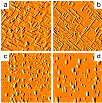
Fig. (7-3): AFM images of the reactive interface (11\bar{2}0)_{ZnO} \parallel (1\bar{1}02)_{sapphire} at increasing heating time at 800 °C: (a) sample heated for 20 minutes; (b) sample heated for 40 minutes; (c) sample heated for 60 minutes and (d) sample heated for 120 minutes
