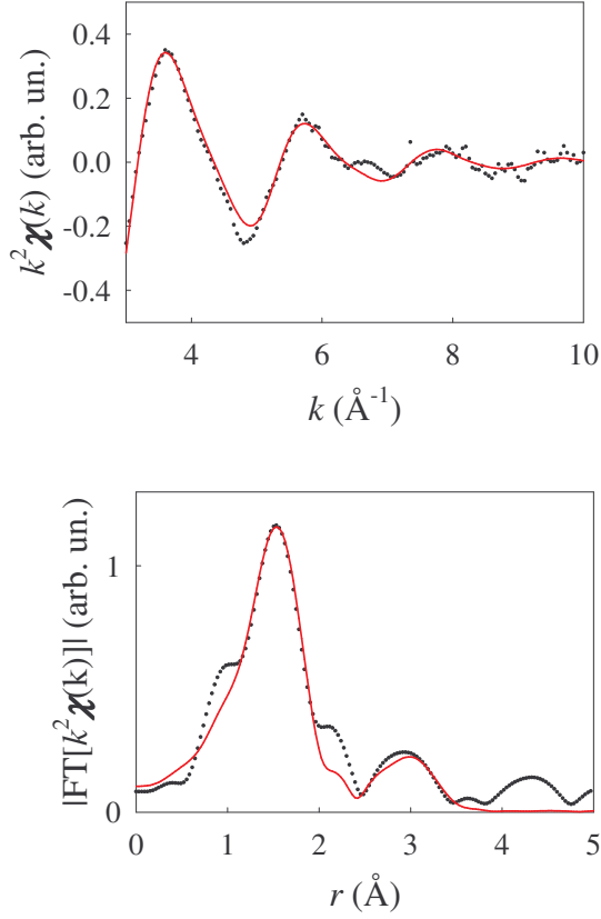
Fig. (4-9): Unpolarised Zn-K edge EXAFS spectra (upper panel) and EXAFS Fourier Transform (lower panel) of the samples investigated in this work. The spectra of powdered ZnO and ZnAl 2 O 4 are also shown for reference. The experimental data are the dotted line while the red line is the fit.
