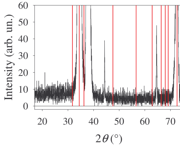
Fig. (3-2): XRPD spectrum of the ZnO thin film deposited at 25 °C onto Al 2 O 3 (11 \bar{2} 0) (black line). For comparison purposes the ZnO reference lines are reported (red bars)
