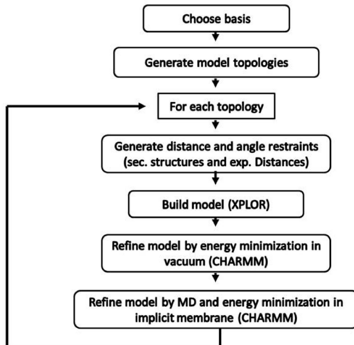
Figure 4.6: Flow chart showing the protocol of model building. A basis is first chosen that is a series of TMHs that will bind the metal and whose topology will be constant in all models. Then model topologies are generated using a homemade C++ program: "buildtopo". Then for each of these models, 3D coordinates are built using X-PLOR and refined using MD simulation with CHARMM inside an implicit membrane after the introduction of 2 Cd 2+ ions.
