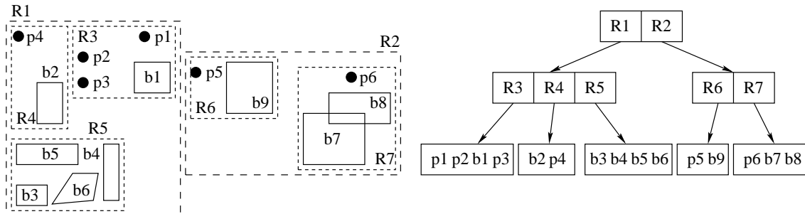
Figure 5.10 – R*-Tree
