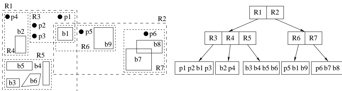
Figure 5.9 – R-Tree
