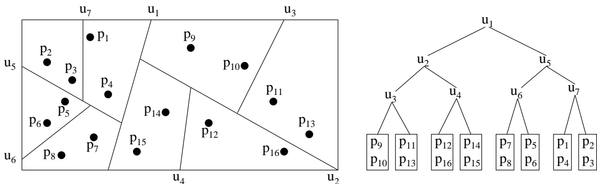
Figure 5.8 – BSP-Tree
