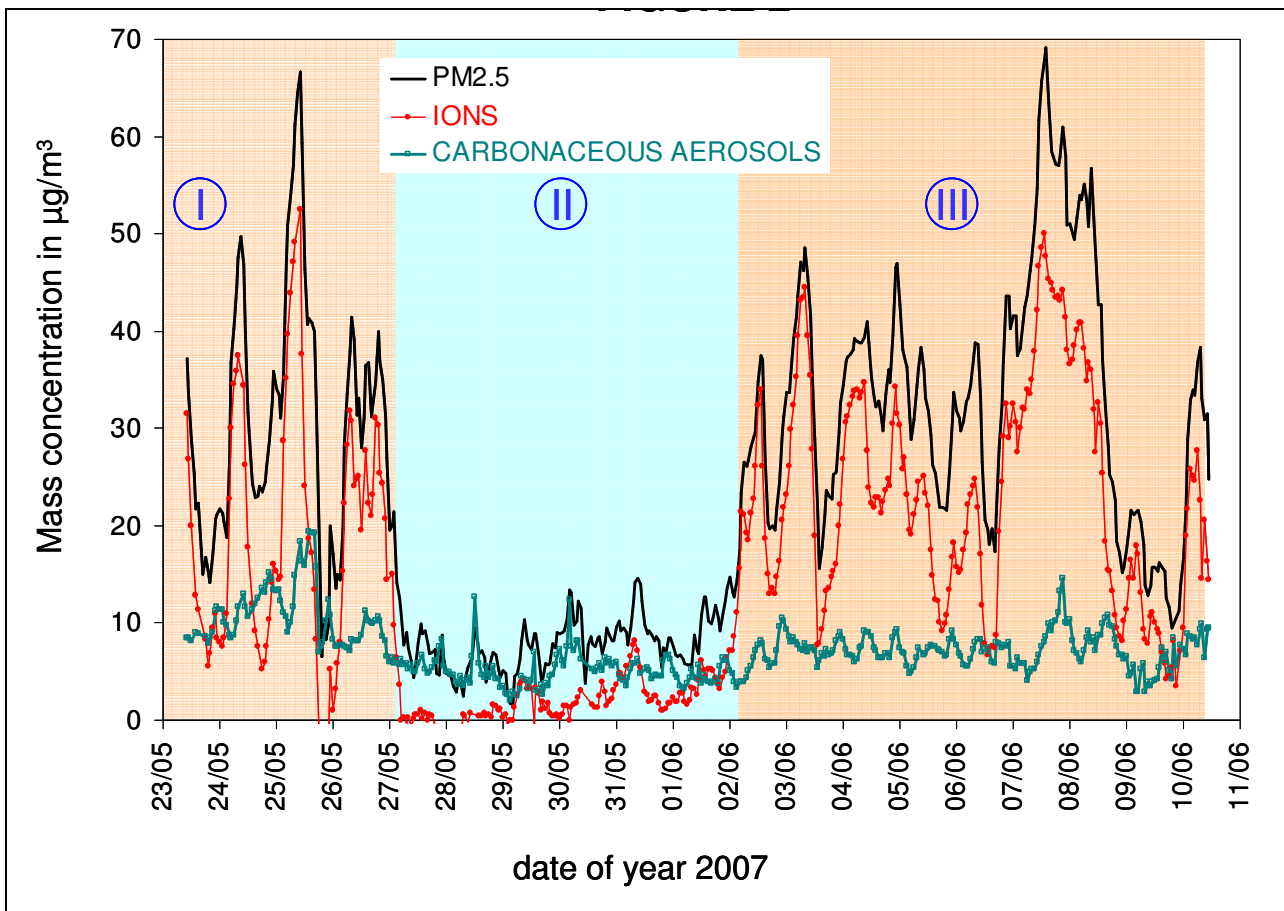
Figure 1 : Comparison between \text{PM}_{2.5} concentrations measured by the TEOM-FDMS and reconstructed from the chemistry by summing BC, POM, and ions (see section 3.2).
