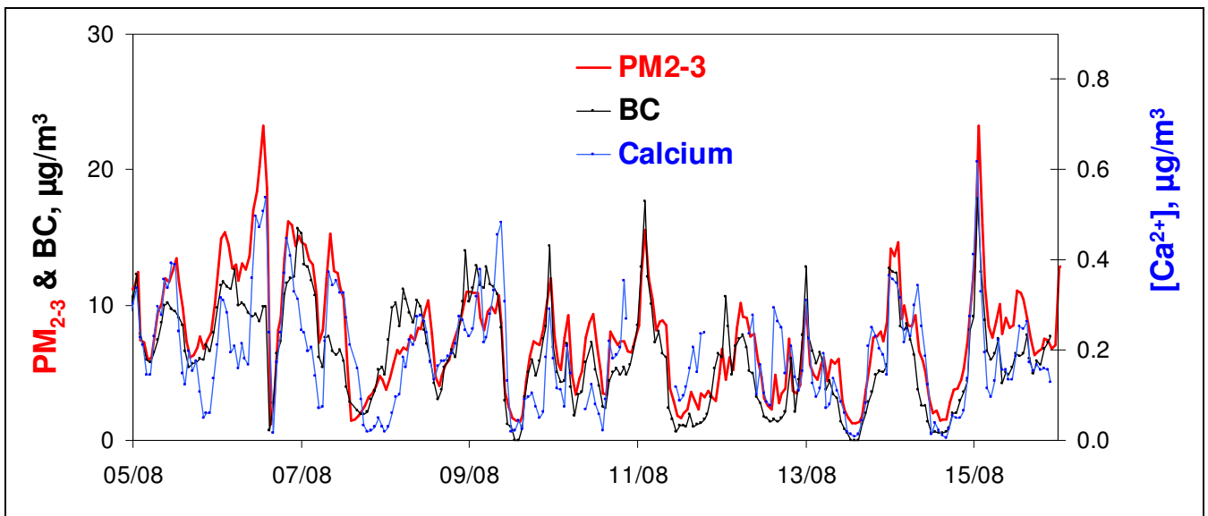
Figure 3: Covariation of real-time PM 2-3 , Ca (PM 2.5 ) and BC (PM 2.5 ) concentrations showing the resuspension origin of dust; (PM 2-3 calculated from Grimm OPC data, Ca from PILS-IC, BC from Aethalometer).
