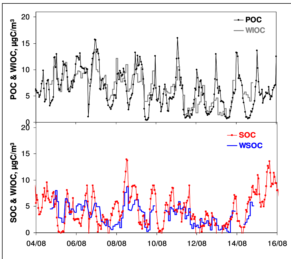
Figure 5: one to two hours quasi real time data for the various OC fractions. 5-A Covariation of primary organic aerosol (POC, calculated with EC tracer method) and WIOC (Calculated as OC-WSOC); 5-B Covariation of secondary organic aerosol (SOC, calculated with EC tracer method) and WSOC.
