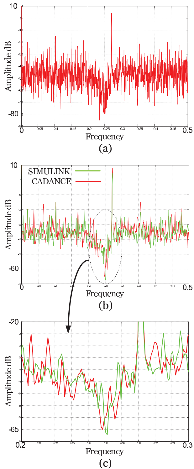
Figure 6.51: Power spectrum density of the modulator output, simulated in layout-level, for 4400 points of the simulation (a) compared with an ideal modulator simulated by SIMULINK, where 1100 points are illustrated (b), for the typical mean value.
