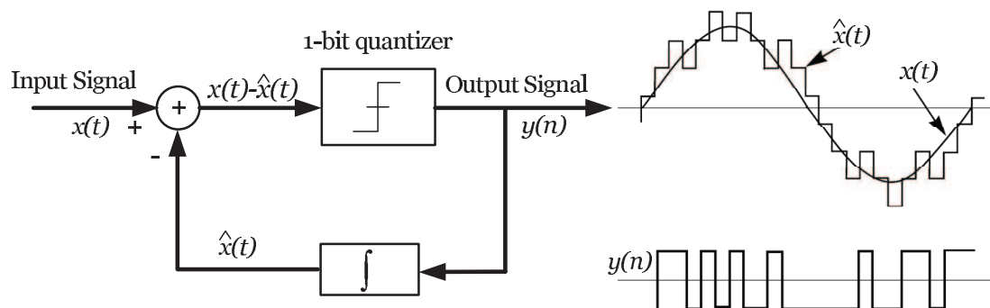
Figure 2.8: Delta modulation principle.
