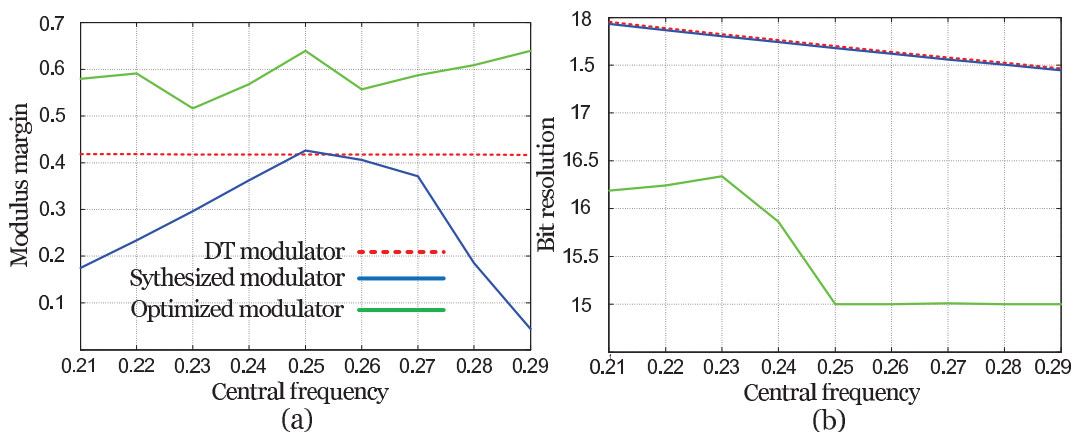
Figure 5.19: Comparison of the modulus margin (a) and the bit resolution of the optimized, synthesized and original DT modulator.
