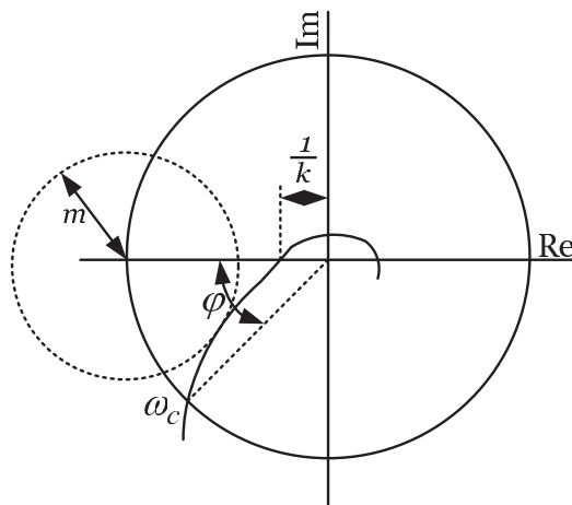
Figure 2.24: Modulus, gain and phase margin for the open-loop frequency characteristic.
