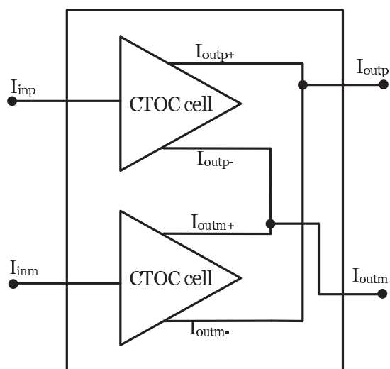
Figure 6.9: Global view of the differential buffer.
