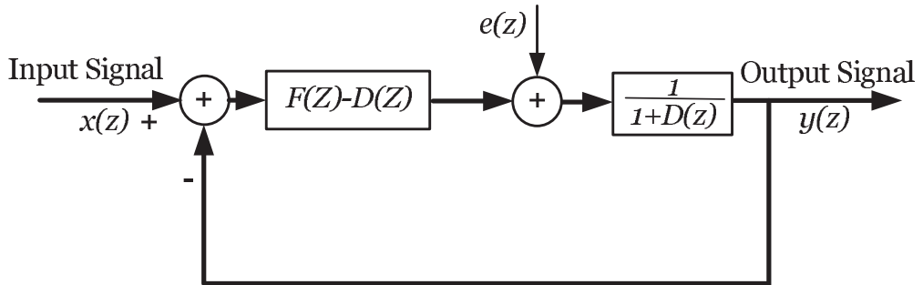
Figure 2.27: First step to find the linear DT mono-loop model.
