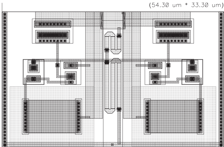
Figure 6.29: Layout of the CTOV circuit.
