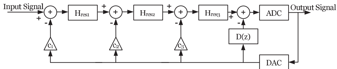
Figure 2.21: 6 th -order mono-feedback structure.
