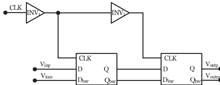
Figure 6.14: Differential flip-flop.
