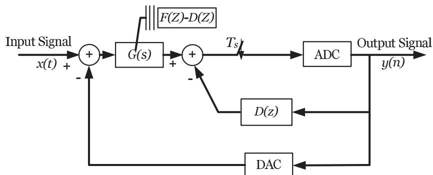
Figure 2.16: A possible implementation of equation 2.13.
