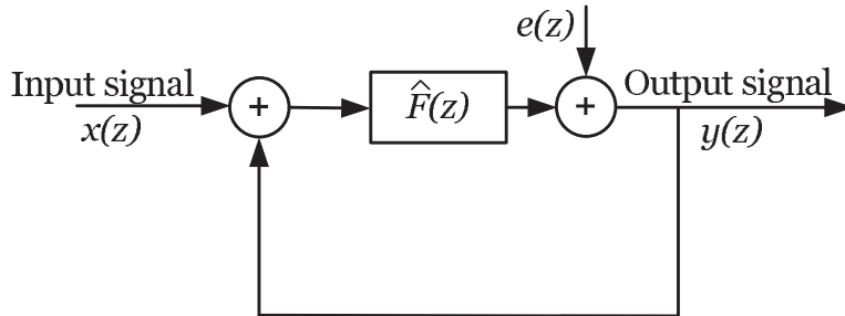
Figure 2.25: Required DT linear model of CT modulators for calculating the stability margins.
