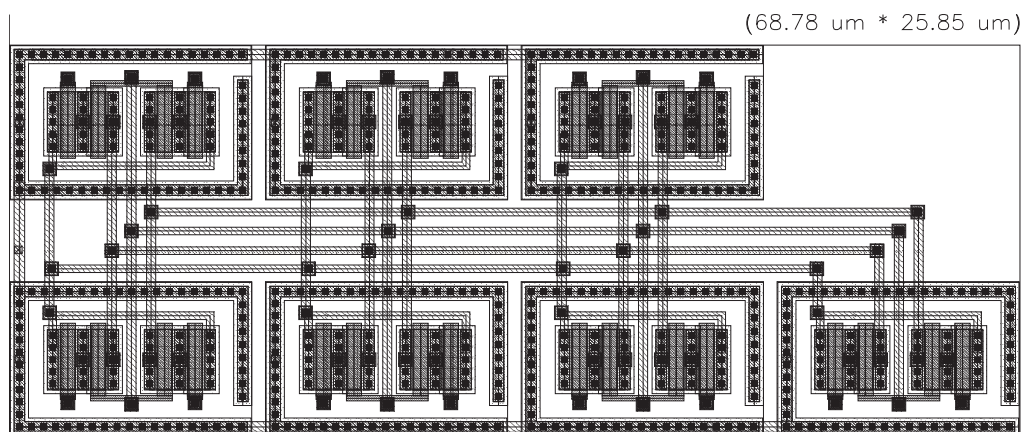
Figure 6.44: Layout of the DAC circuit.
