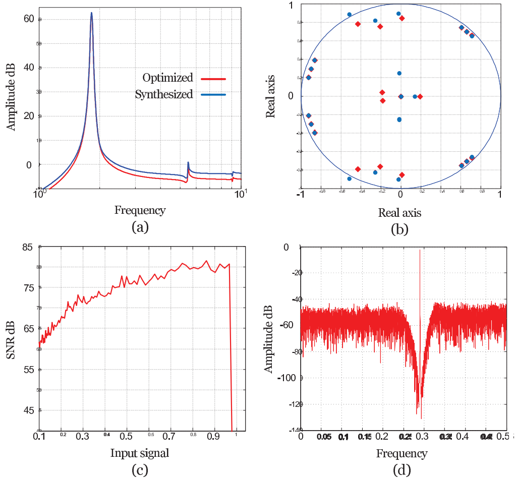
Figure 5.29: G(s) (a) and the position of the NTF poles (b) for optimized and non optimized modulator. The SNR (c) and the output signal spectrum (d) for f_c = 0.29f_s .
