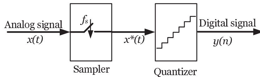
Figure 2.1: Analog-to-digital conversion.
