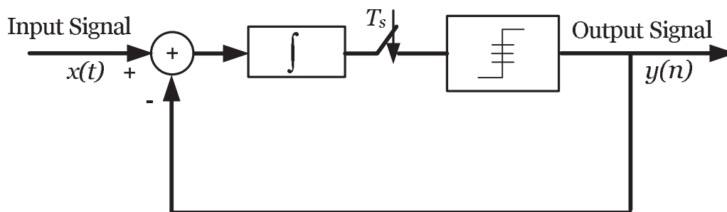
Figure 2.9: \Sigma\Delta modulation.
