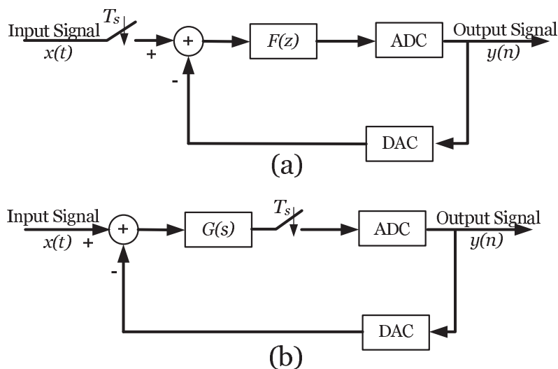
Figure 2.13: DT \Sigma\Delta modulator structure (a), CT \Sigma\Delta modulator structure (b).
