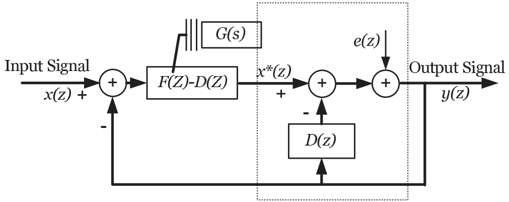
Figure 2.26: Another representation of figure 2.16 .
