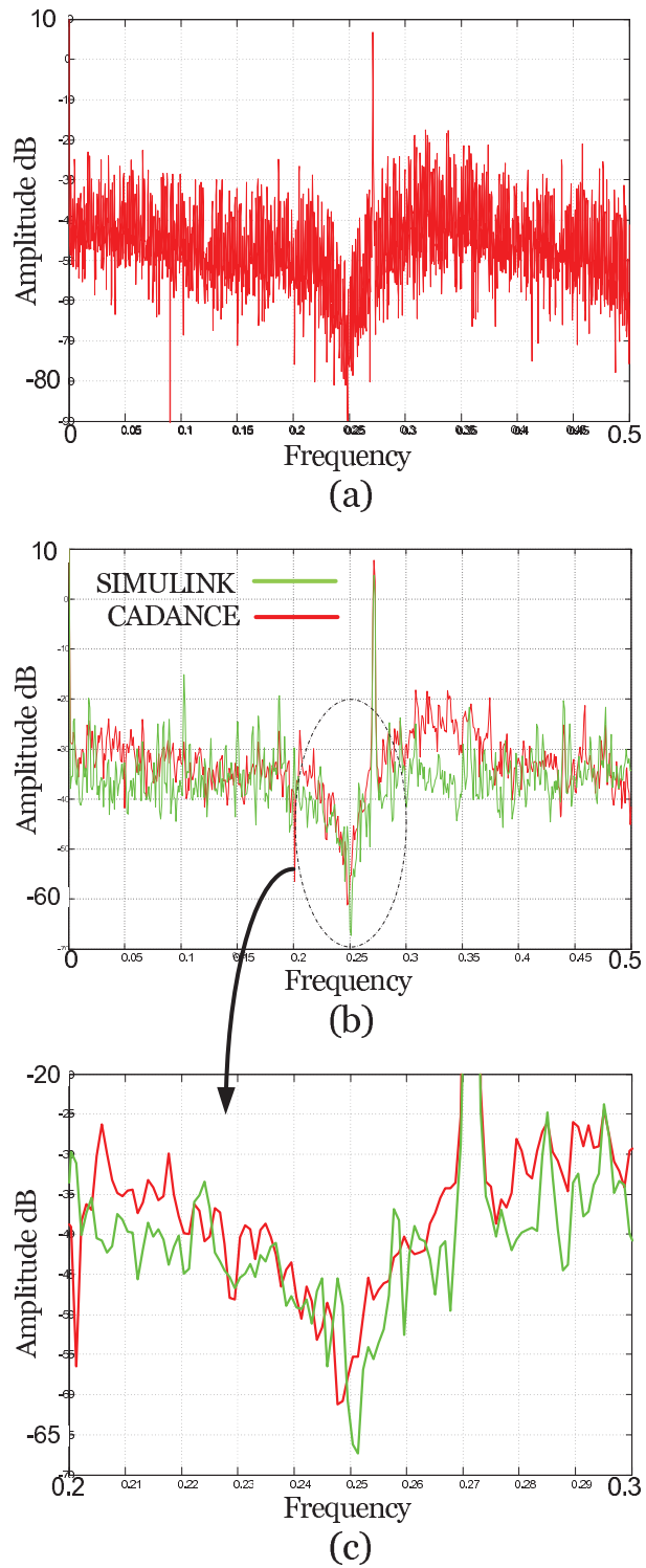
Figure 6.53: Power spectrum density of the modulator output, simulated in layout-level, for 4400 points of the simulation (a) compared with an ideal modulator simulated by SIMULINK, where 1100 points are illustrated (b), for the second worst case of the design.
