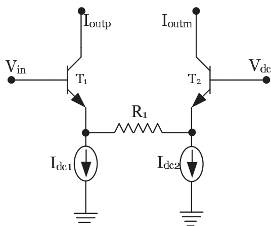
Figure 6.5: Schematic of the voltage to current converter.
