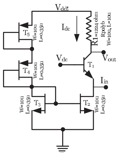
Figure 6.3: Benchmark schematic to test the influence of the worst cases.
