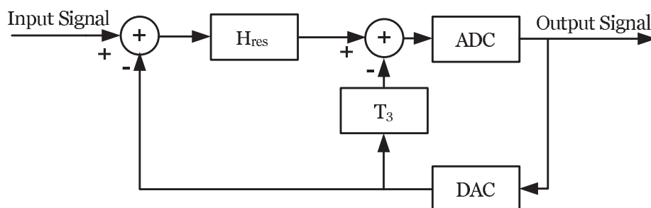
Figure 6.22: Second-order single-stage \Sigma\Delta modulator.
