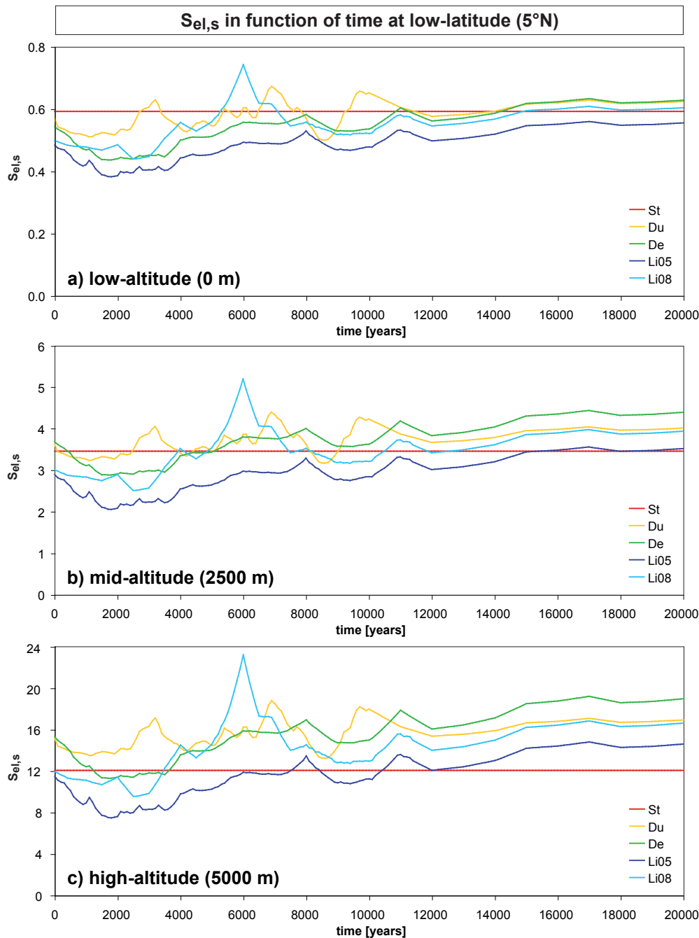
Figure 1.17: The scaling factor S_{el,s} for spallation reactions in function of time (0 - 20 ka) at low-latitude ( 5^{\circ}N ) for (a) low-altitude (0 m), (b) mid-altitude (2500 m) and (c) high-altitude (5000 m). Note that the scales of the axes of ordinates are different for each panel. The abbreviations in the legend represent the following scaling methods: St = Stone (2000), Du = Dunai (2001), De = Desilets et al. (2006b), Li05 = Lifton et al. (2005), Li08 = Lifton et al. (2008). In the case of Du, for the first 10 ka, non-dipole components are considered based on the paleoinclination record of Brandt et al. (1999) from 42.5^{\circ}N (Italy).
