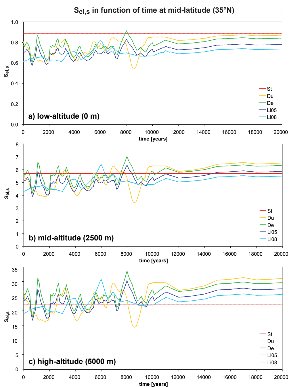
Figure 1.18: The scaling factor S_{el,s} for spallation reactions in function of time (0 - 20 ka) at mid-latitude ( 35^{\circ}N ) for (a) low-altitude (0 m), (b) mid-altitude (2500 m) and (c) high-altitude (5000 m). Note that the scales of the axes of ordinates are different for each panel. The abbreviations in the legend represent the following scaling methods: St = Stone (2000), Du = Dunai (2001), De = Desilets et al. (2006b), Li05 = Lifton et al. (2005), Li08 = Lifton et al. (2008). In the case of Du, for the first 10 ka, non-dipole components are considered based on the paleoinclination record of Brandt et al. (1999) from 42.5^{\circ}N (Italy).
