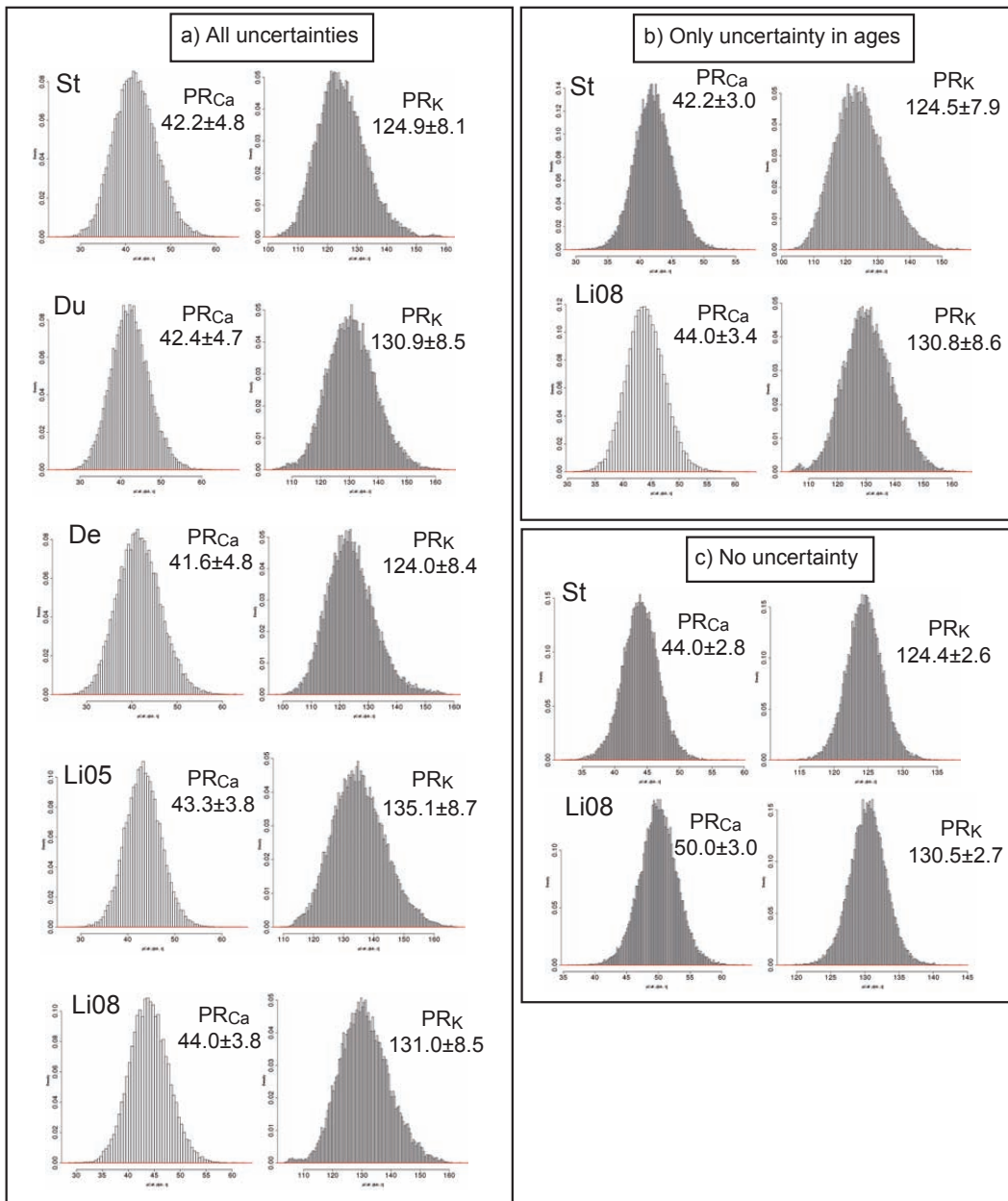
Figure 5.7: Posterior distributions of PR_{Ca} and PR_K resulting from the Bayesian statistical analysis of the calibration data set. (a) All uncertainties in the selected parameters t_{expo} , P_\mu and \varepsilon are integrated. (b) Only the uncertainty in t_{expo} of each flow is considered. (c) No uncertainties are assigned to the parameters. In (b) and (c), only the distributions for the results when using the scaling methods of St and Li08 are illustrated. This choice was made because the new "St" production rates are among the lowest mean values, while the new "Li08" production rates are among the highest mean values.
