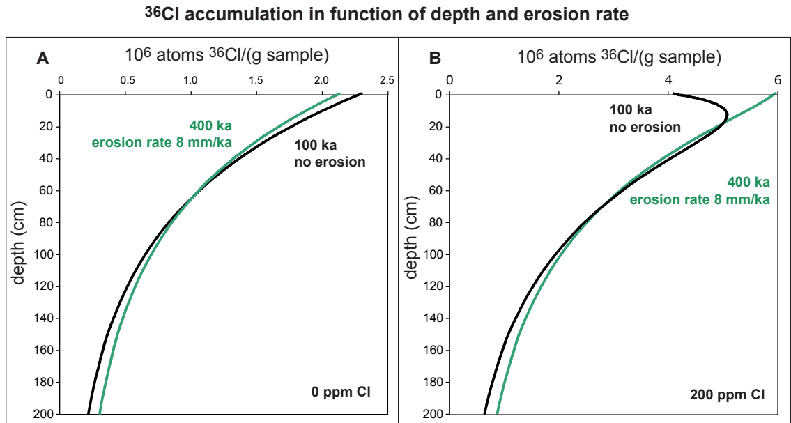
Figure 3.6: Vertical distributions of theoretical ^{36}\text{Cl} concentrations in a basalt sample at 2000 m altitude: In panel A it is assumed that the sample has 0 ppm Cl, 8.9% Ca and 0.6% K. ^{36}\text{Cl} production is therefore dominated by spallation reactions (by 93%), responsible for the exponential shape of the curve. In panel B it is assumed that the same sample has 200 ppm Cl, which results in a ^{36}\text{Cl} contribution from capture of low-energy neutrons of 57%. This explains the characteristic shape of the black curve with a peak of maximum ^{36}\text{Cl} production at a about 15 cm depth, which is due to neutron leakage back into air near the land/atmosphere boundary. When a depth profile is measured and both exposure age and erosion rate are to be determined (see paragraph "Depth profile" in this section), this characteristic shape can help identifying the values for the two free parameters with less ambiguities than if production is dominated by spallation. In panel A, two very similar theoretic vertical distributions can be explained by very different exposure age/erosion rate combinations. In panel B, on the other hand, the same exposure age/erosion rate combinations result in clearly different shapes of the theoretical profile. The form of the curves changes in panel B, because in the case of erosion, layers of the material are steadily removed from the surface while ^{36}\text{Cl} production continues at the same rate. This can be imagined as if deeper parts of the curves were uplifted to the surface, which explains why the peak of maximum production in panel B has moved to the surface.
