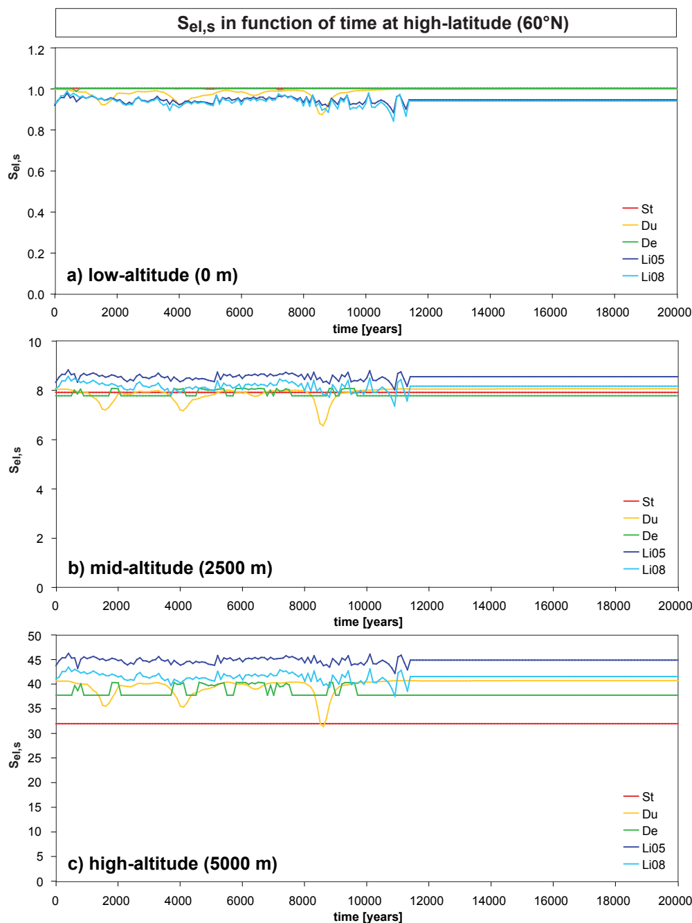
Figure 1.19: The scaling factor S_{el,s} for spallation reactions in function of time (0 - 20 ka) at high-latitude ( 60^\circ N ) for (a) low-altitude (0 m), (b) mid-altitude (2500 m) and (c) high-altitude (5000 m). Note that the scales of the axes of ordinates are different for each panel. The abbreviations in the legend represent the following scaling methods: St = Stone (2000), Du = Dunai (2001), De = Desilets et al. (2006b), Li05 = Lifton et al. (2005), Li08 = Lifton et al. (2008). In the case of Du, for the first 10 ka, non-dipole components are considered based on the paleoinclination record of Brandt et al. (1999) from 42.5^\circ N (Italy).
