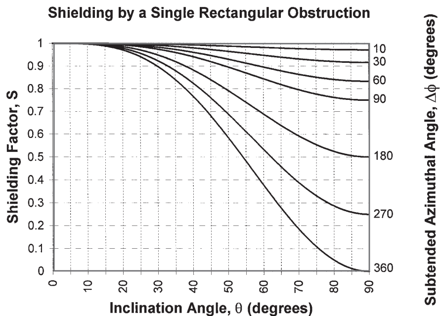
Figure 1.9: Shielding factor that results from a rectangular obstruction screening a surface from cosmic rays, depending on the inclination angle (angle in vertical direction between horizontal and top of the obstruction, measured from the sample site) and the azimuthal angle (angle between the two endpoints of the obstruction in the horizontal plane) (from Dunne et al., 1999). A factor of 1 means no shielding, while a factor of 0 means complete shielding.
