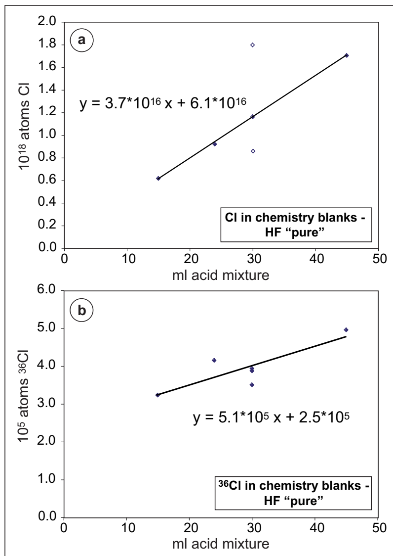
Figure 4.2: Absolute number of (a) atoms Cl and (b) atoms 36 Cl in chemistry blanks versus ml of acid mixture (one part HF, "pure", 48%, two parts HNO 3 , 2M). Open symbols are considered as outliers. The linear relationship indicates that HF "pure" contains significant amounts of Cl and 36 Cl. See text in section 4.2.2 for details.
