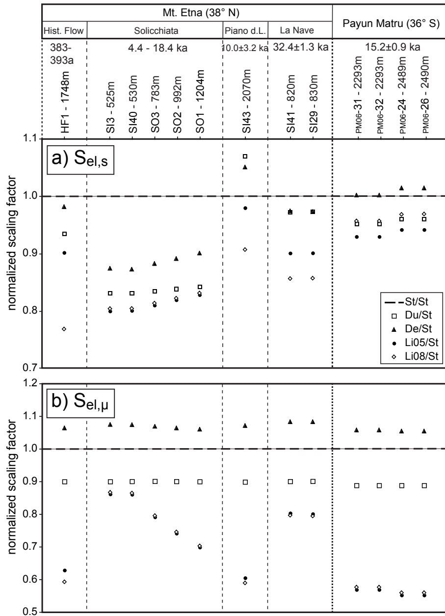
Figure 5.6: Normalized scaling factors for spallation reactions (a) and slow negative muon capture (b) for each calibration site according to the five different scaling methods. Scaling factors derived from Du, De, Li05 and Li08 are normalized to those derived from St to display the differences between the methods in function of the altitude of the sample site and the exposure duration of the flows. Absolute values are listed in Table C.1. In the case of the four methods that consider temporal variations (Du, De, Li05 and Li08), the scaling factors were integrated over the following time spans: Historical Flow 0-400 years, Solicchiata 0-8 ka, Piano della Lepre 10-20 ka, La Nave 0-32 ka, Payun Matru 0-15 ka.
