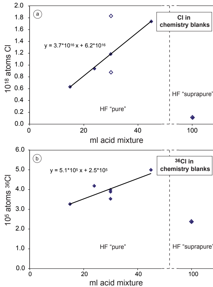
Figure 2.12: Absolute numbers of (a) atoms Cl and (b) atoms 36 Cl in chemistry blanks versus ml of acid mixture (one part HF, conc., two parts HNO 3 , 10%). On the left side of both plots, HF brand Chimie-Plus Laboratoires reagent grade "pure" was used, on the right side, HF brand MERCK "suprapur ® " was used. The linear relationship on the left side indicates that HF "pure" contains significant amounts of Cl and 36 Cl. Open symbols are considered as outliers. In this case, the blank correction of the sample has to be done in function of the amount of acid used to dissolve the sample.
