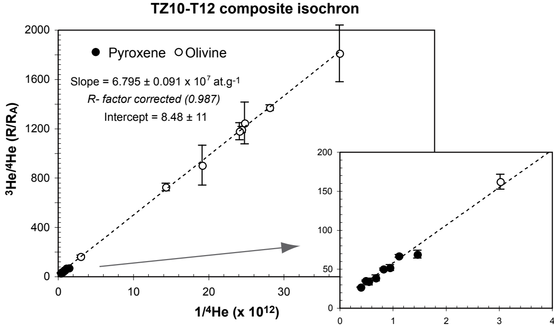
Figure 6.5: Isochron plot of helium concentrations in olivine and pyroxene of samples TZ10 and TZ12. The intercept represents the magmatic ({}^3\text{He}/{}^4\text{He})_{\text{mag}} ratio, and the slope the cosmogenic {}^3\text{He} concentration.
