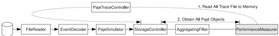
Figure 5.2 – Organization of Performance Tests developed with Pajé components.
