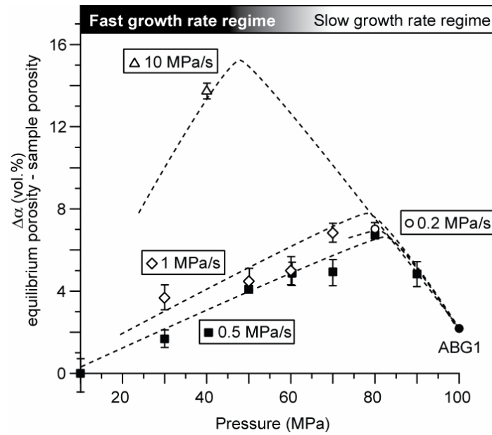
Figure 5 Porosity deviation from equilibrium degassing ( \Delta\alpha ) for various linear decompression rates. The y-axis corresponds to the degree of super-saturation and dashed lines to the regressions used in the model. Regressions were carried out using the linearity of the slow growth regime and the assumption that super-saturation vanishes at atmospheric pressure (see text). Error bars are omitted when smaller than the symbol size.
