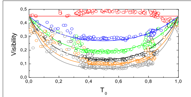
FIGURE 7.18 – (color online) Visibility decrease of the interferometer as a function of T_0 for V_2=0, 21, 31, 42, 53 and 63 \mu\text{V} from top to bottom. The solid lines are fits to the data using Eq. 1 with V_0=0.45 , V_\varphi = 7.2\mu\text{V} and T=25\text{mK} .
